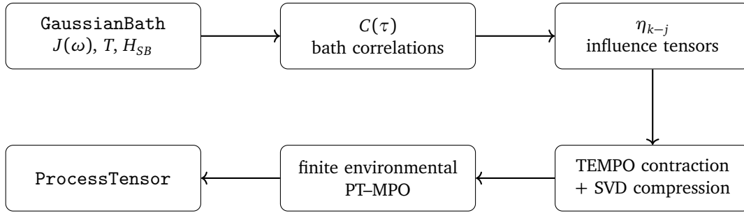
Figure 18: Proposed PT-TEMPO construction in the present package. A stationary Gaussian bath is specified directly through its spectral density, temperature, and system–bath coupling. The corresponding two-time correlations generate the discretised Feynman–Vernon influence tensors, which are contracted and compressed into a finite environmental PT-MPO. Free-system propagation is then embedded using the same convention as the existing process-tensor builders, producing the standard ProcessTensor object used by the rest of the package.
