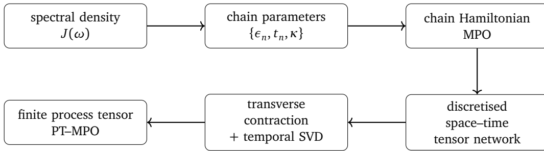
Figure 19: Prospective chain-mapping route from a continuum spectral density to a finite temporal PT-MPO.
