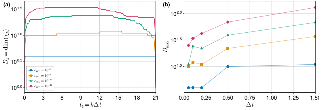
Figure 15: Temporal compressibility of the unpolarised central-spin process tensor. (a) Internal bond dimensions along the temporal MPO for several relative cutoffs. (b) Maximum internal bond dimension versus timestep and cutoff. Open symbols indicate runs limited by maxdim; the bath realisation is fixed across all points.
