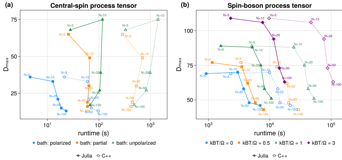
Figure 17: Benchmark of ProcessTensors.jl against the original C++ ACE toolkit. (a) Central-spin baths with fully polarised, partially polarised, and unpolarised initial states. (b) Lorentzian spin–boson baths at four different temperatures. Filled symbols denote Julia and open symbols C++; labels give the number N of bath modes. The horizontal axis is measured PT-MPO construction time and the vertical axis is the maximum internal bond dimension D_{\max} . Vertical alignment of matched points indicates equal retained bond dimension.
