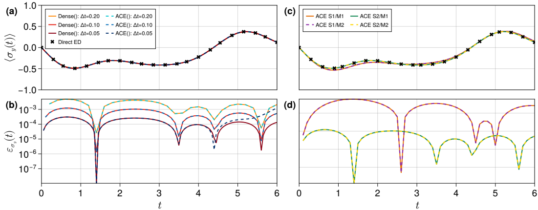
Figure 14: Correctness and propagation errors for the four-mode spin bath. Panel (a) shows the system-spin observable \langle \sigma_y(t) \rangle from direct ED, uncompressed Dense() , and ACE() for three different \Delta t values; panel (b) shows their absolute errors relative to ED. Panels (c,d) compare first- and second-order system and mode-combination splittings at fixed \Delta t .
