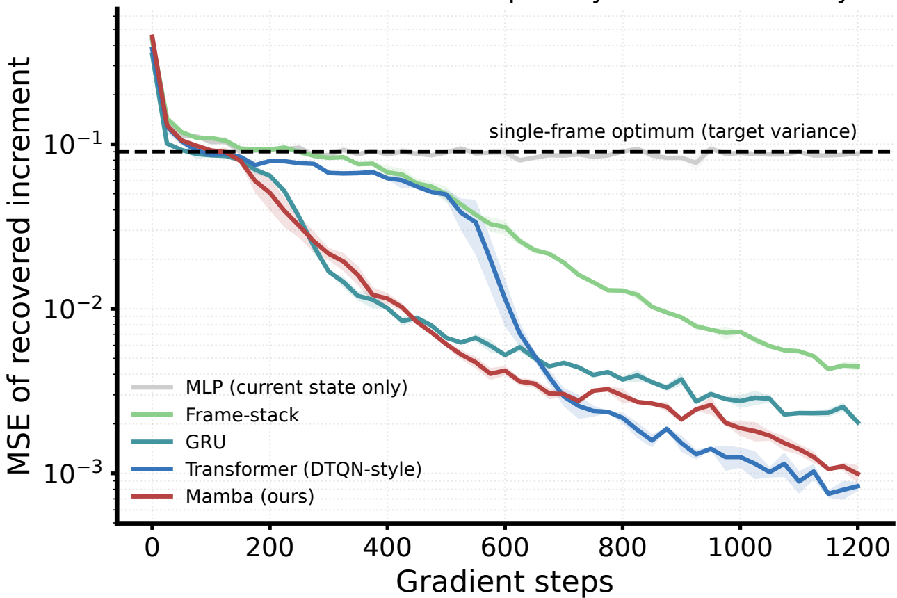
Can the encoder recover a quantity that needs history?
