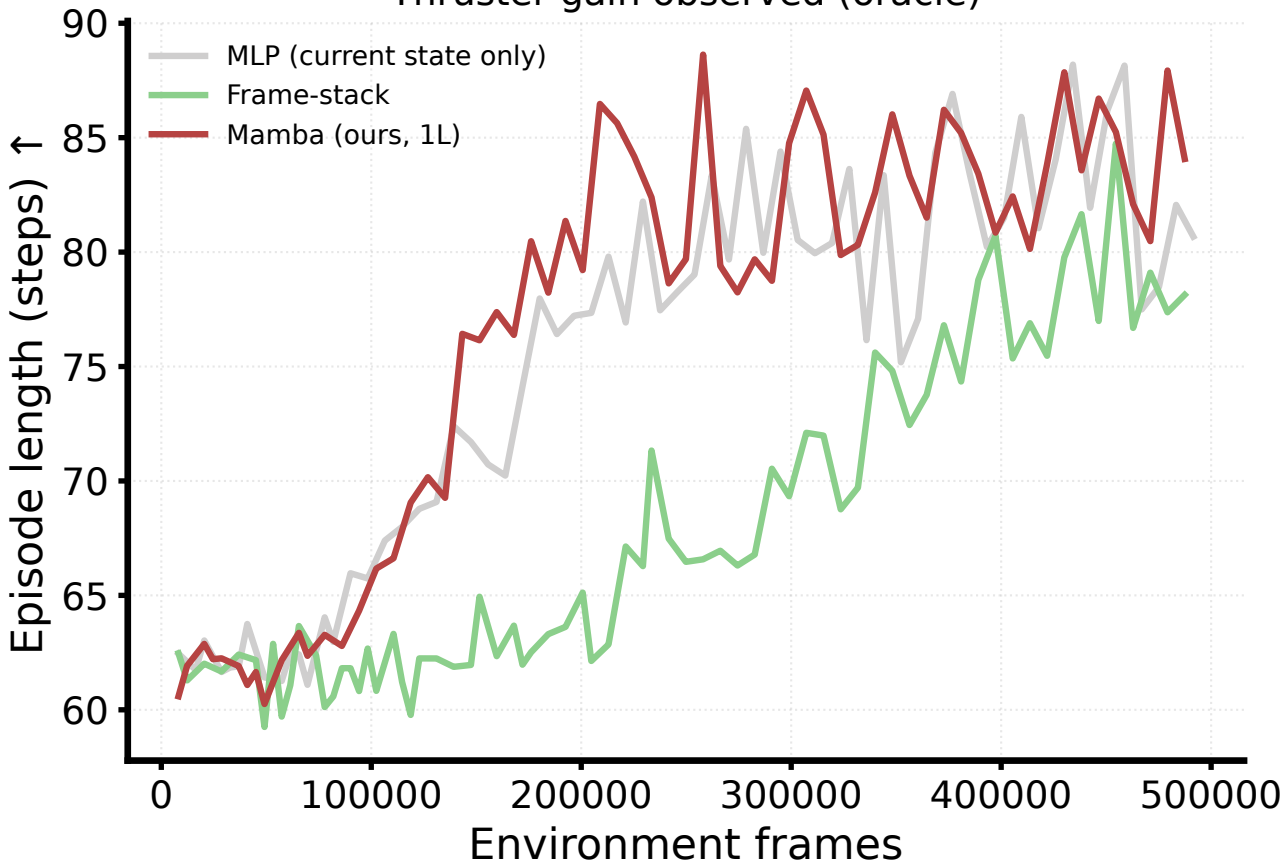
Thruster gain observed (oracle)
