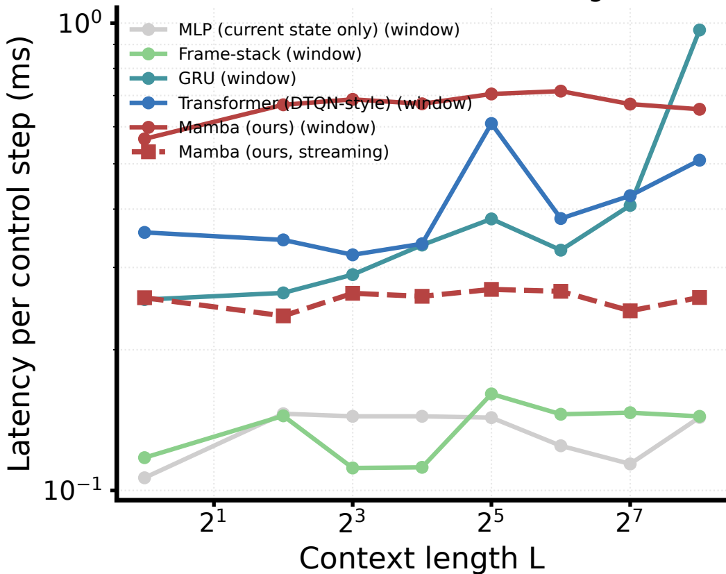
Inference cost vs context length
