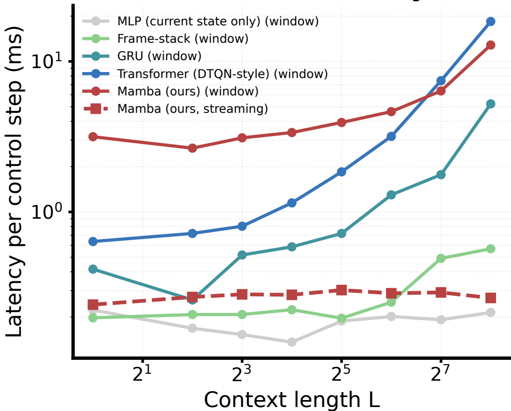
Inference cost vs context length
