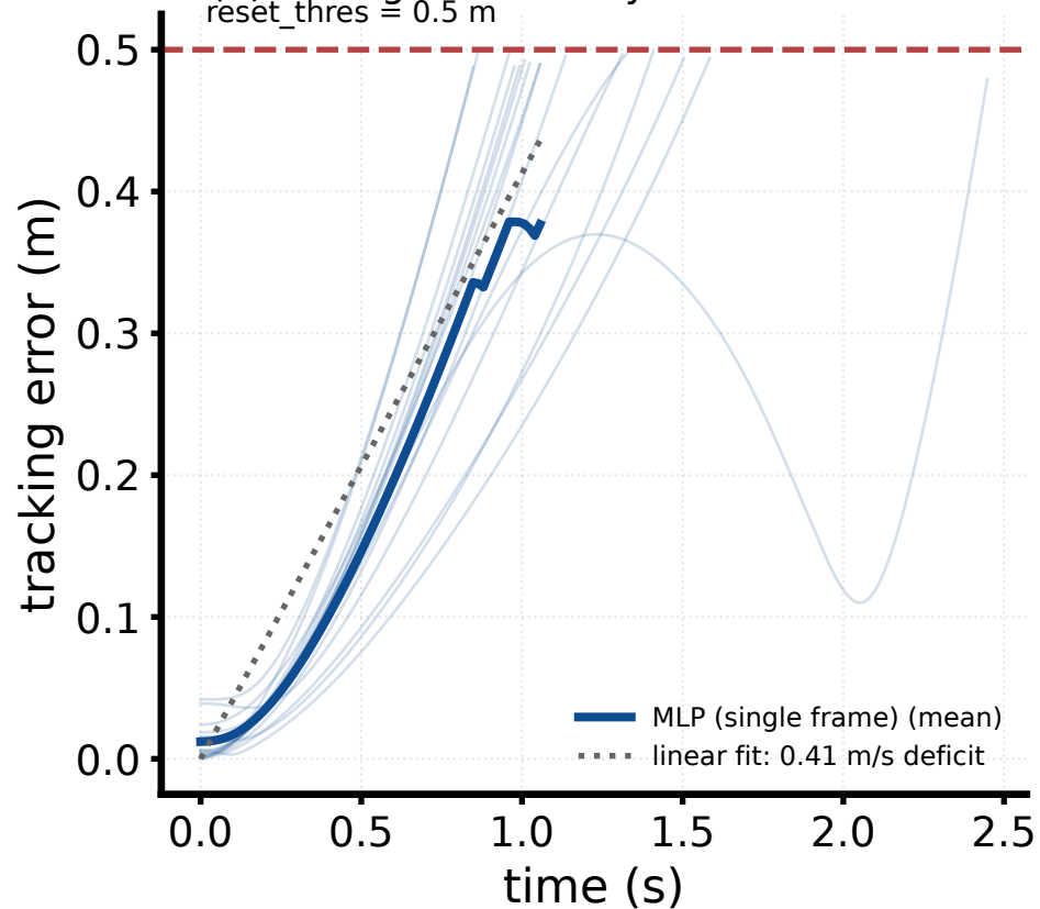
(b) Error grows linearly until termination reset_thres = 0.5 m
