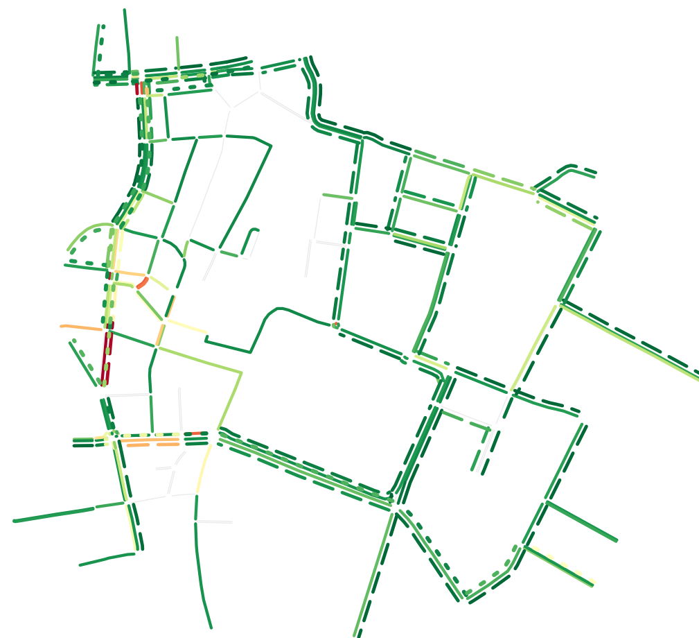
Priority-RL (exp208, 5:3:1)
