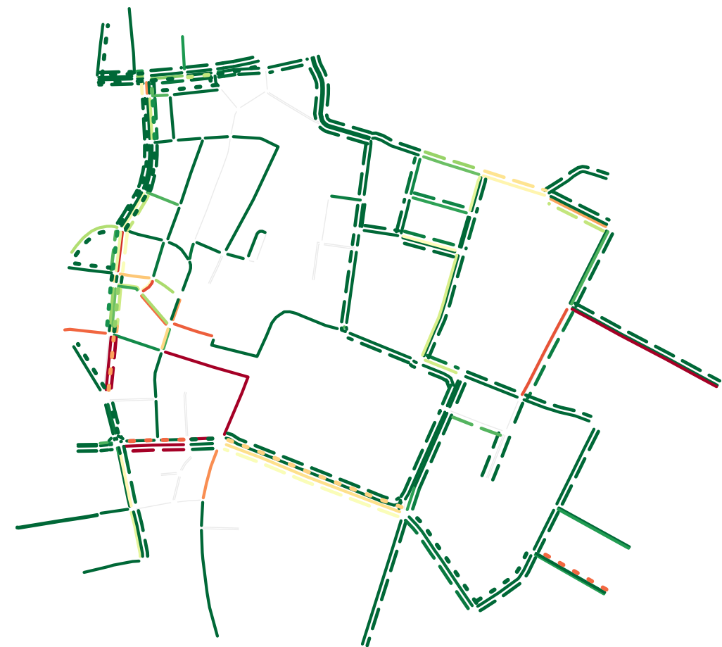
Priority-RL (exp208, 5:3:1)
