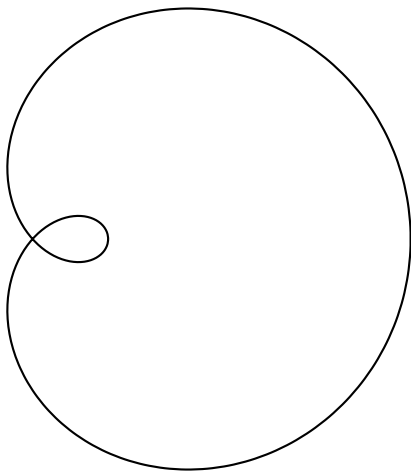
Figure: Task 2: Circle Concoid
