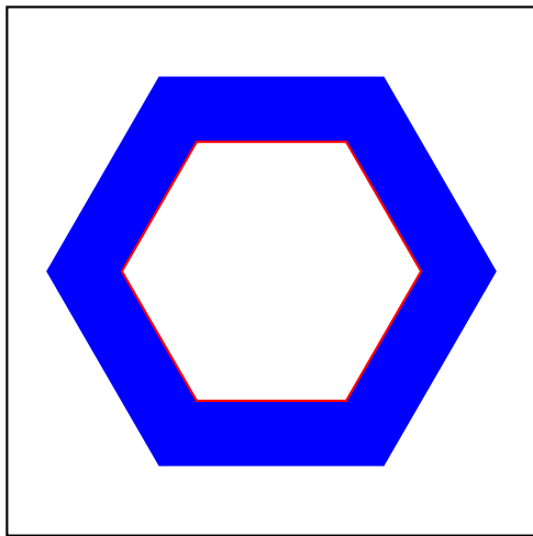
Figure: Task 1: Hexagon drawing
