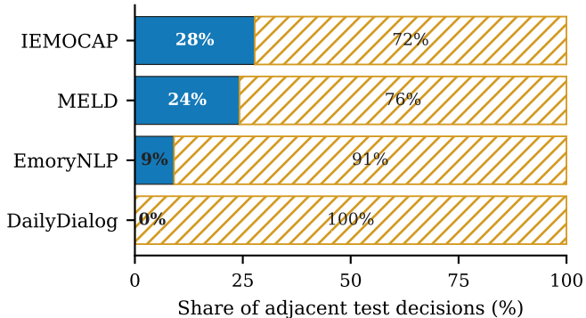
(a) Next-speaker composition
