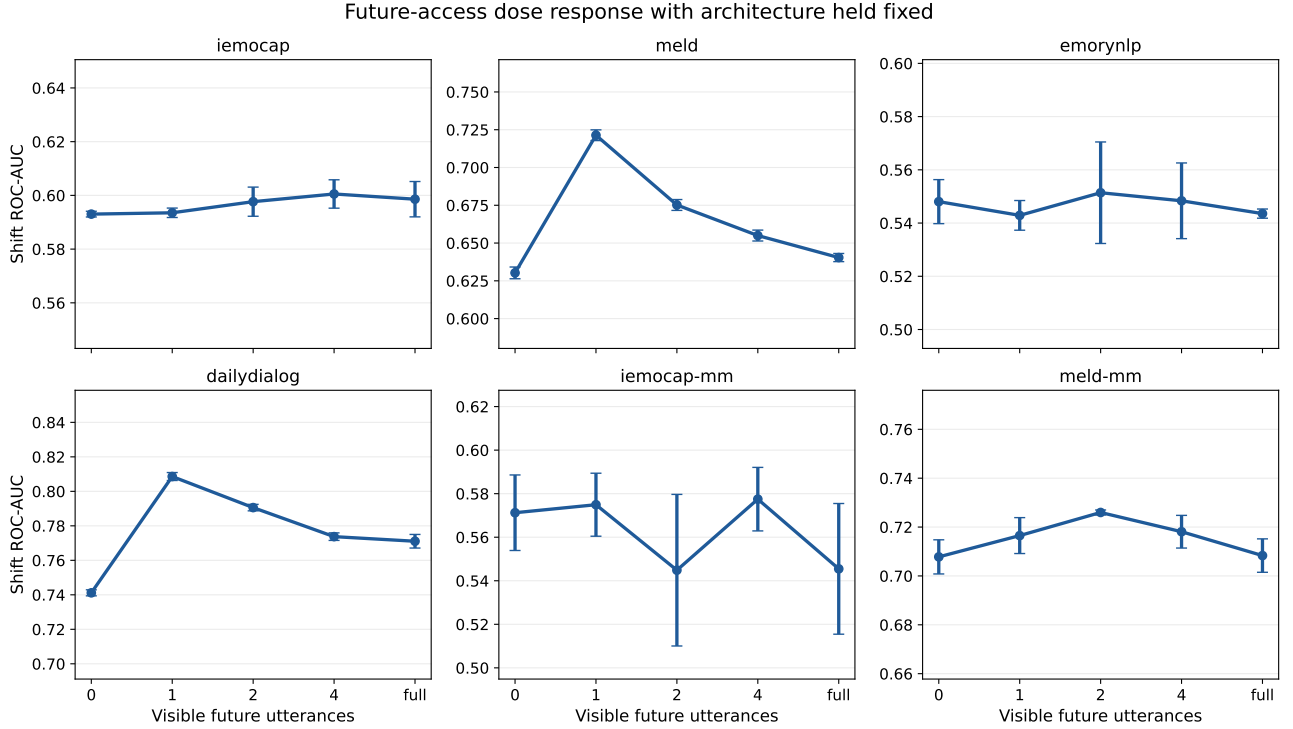
FIGURE 2. Future-access dose response with one fixed Transformer architecture. Error bars show three-seed standard deviation. MELD and DailyDialog peak when the target utterance alone becomes visible; none of the six configurations supports a general monotonic-more-future claim.
