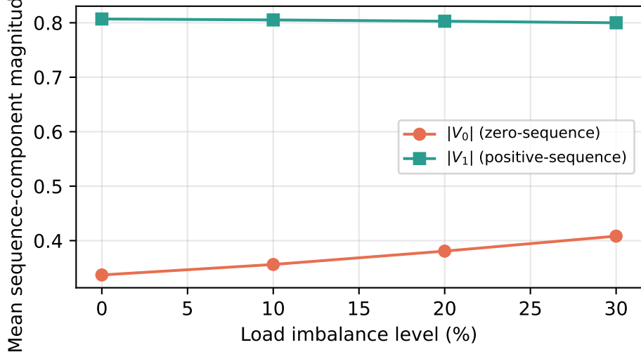
IEEE 13-bus: zero- vs. positive-sequence response to load imbalance
