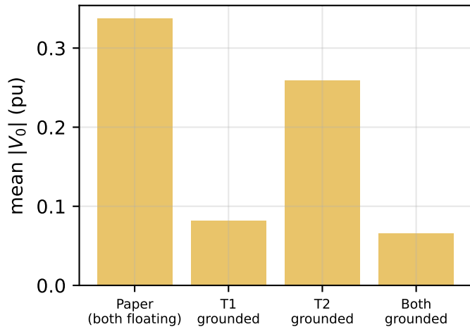
Zero-sequence magnitude
