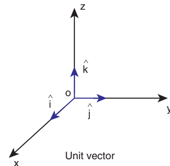
Figure 2.15 Orthogonal unit vectors
