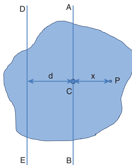
Figure 5.25 Parallel axis theorem
