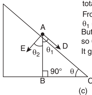
Figure 3.13 (a) Free body diagram, (b) mg resolved into parallel and perpendicular components (c) The angle \theta_2 is equal to \theta
