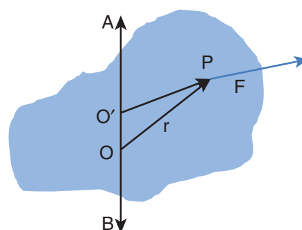
Figure 5.10 Torque about an axis is independent of origin
