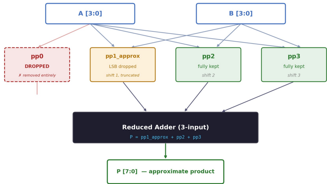
Figure 5.1 – Approximate Multiplier Block Diagram: pp0 dropped, pp1 truncated, pp2/pp3 kept, reduced adder produces P
