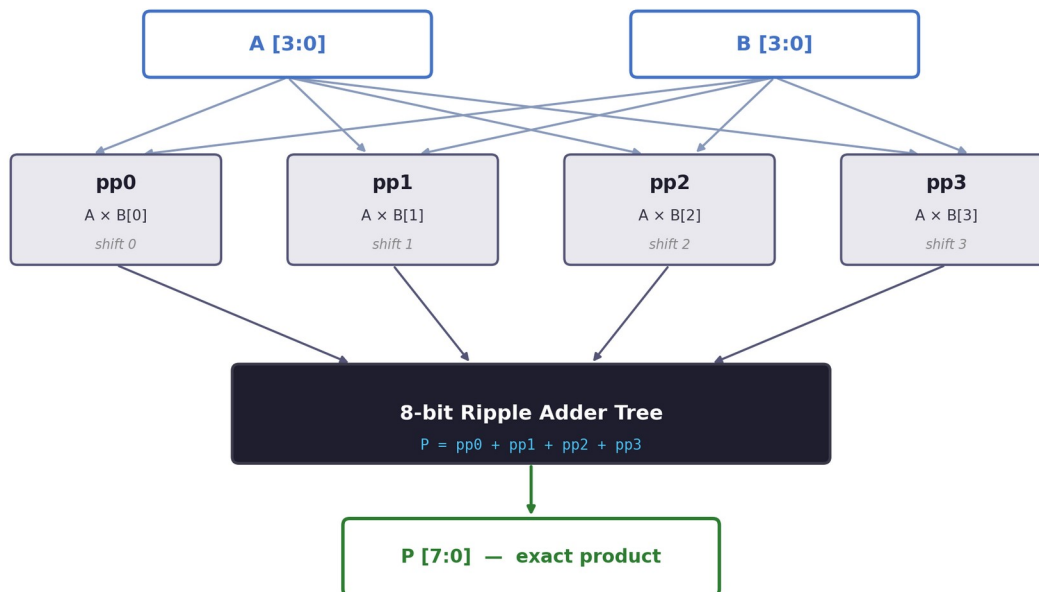
Figure 4.1 – Exact Multiplier Block Diagram: partial products pp0 – pp3 summed by the adder tree to form P
