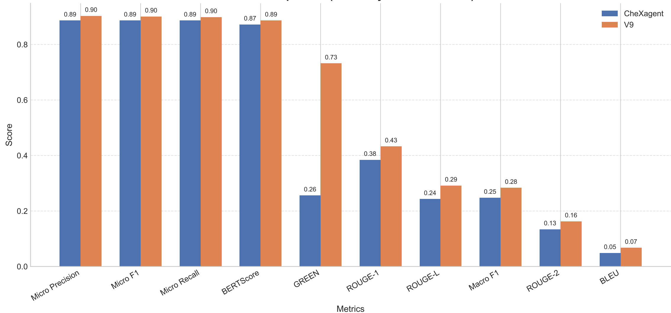
Model Comparison (Sorted by V9 Performance)
