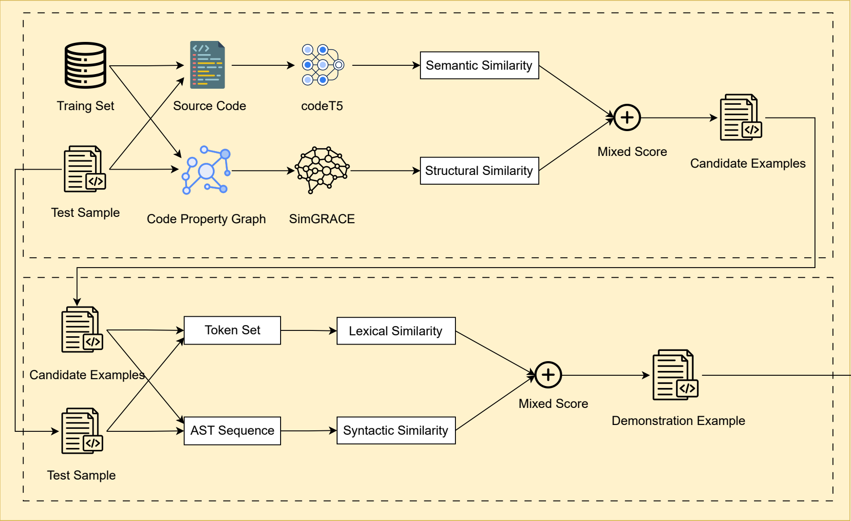
(B) Demonstration Selection Module
