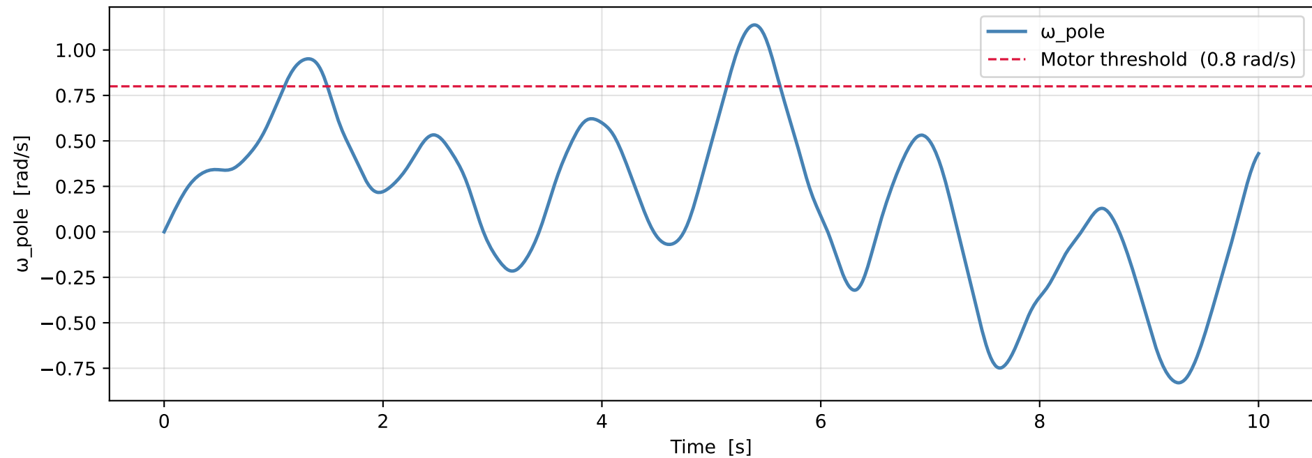
Main Pole — Angular Velocity about I_3
