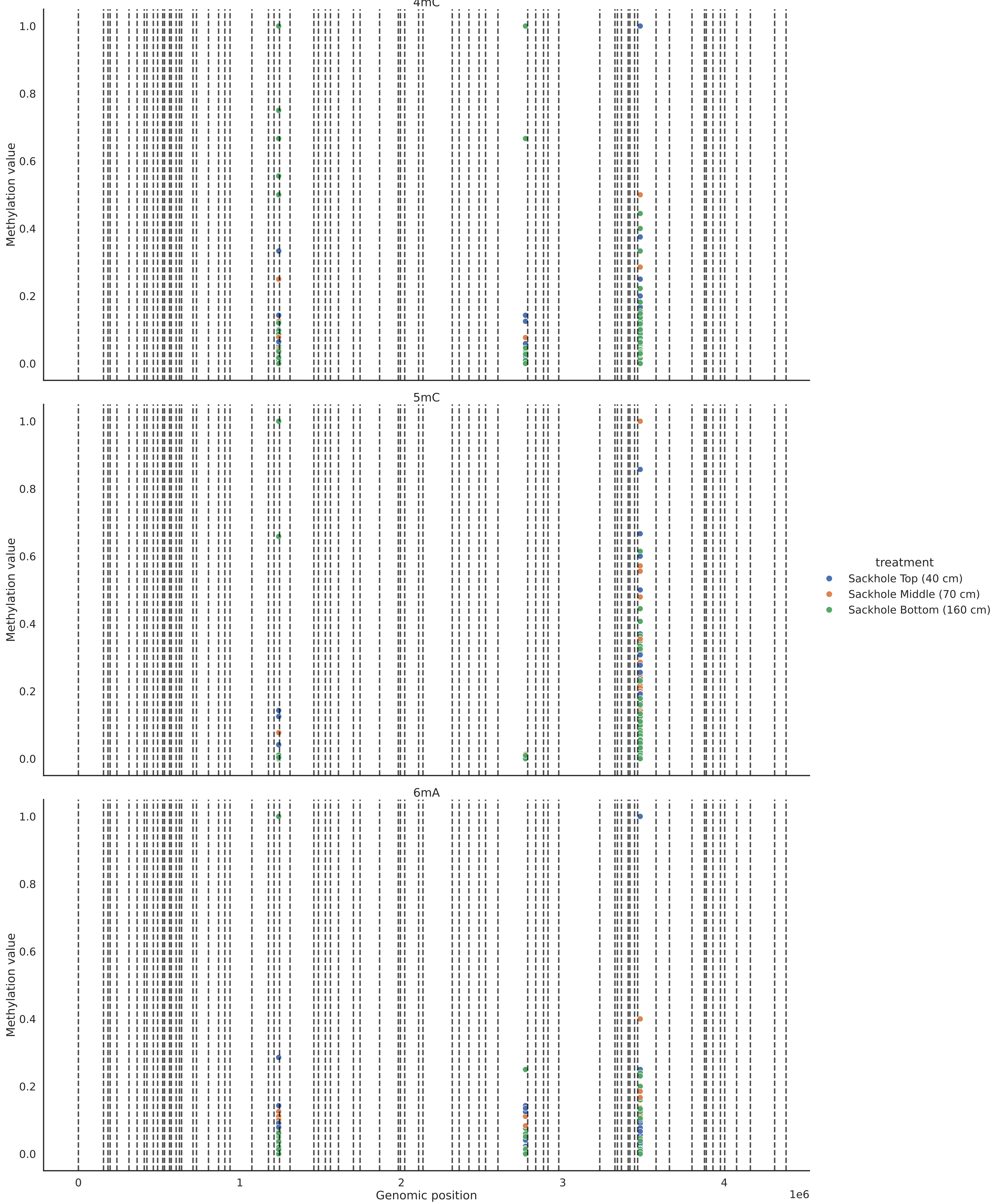
Methylation value across genome of common positions in Rubritalea sp. coverage 7
