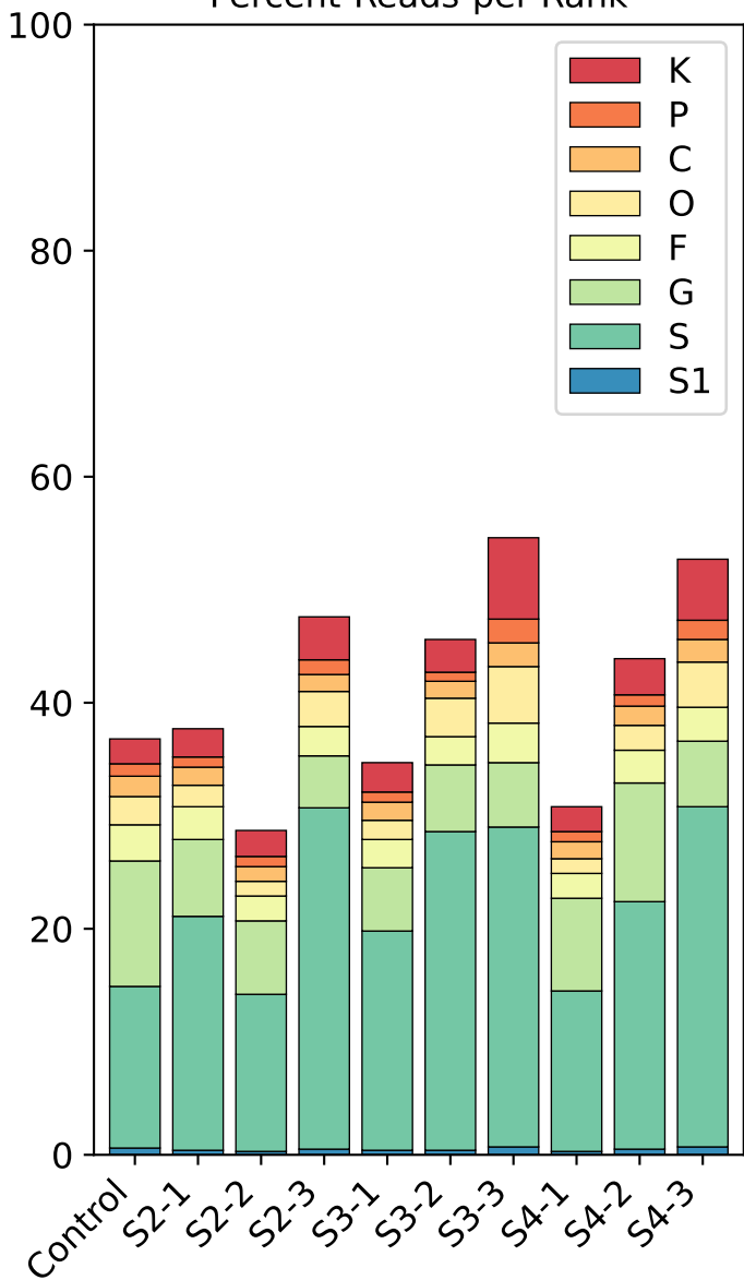
Percent-Reads-per-Rank
