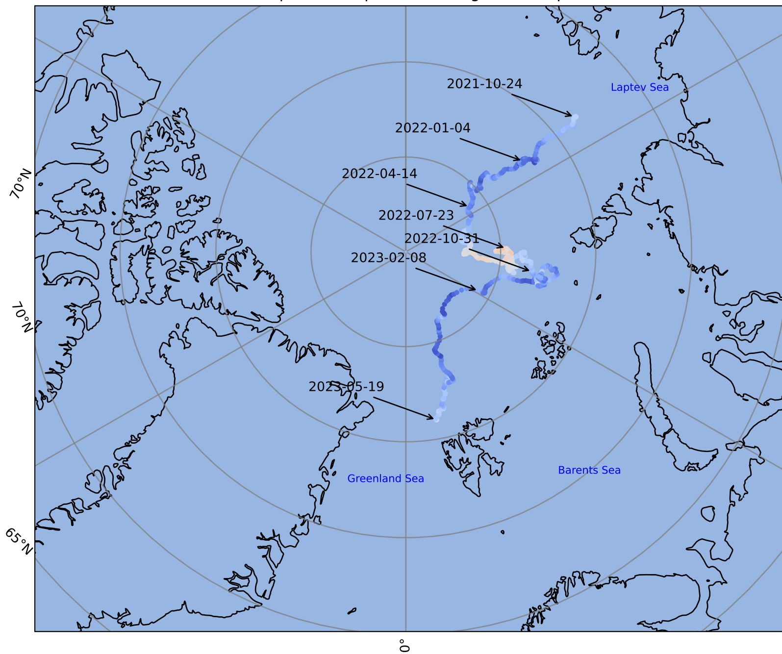
Atmospheric temperature along floe drift path
