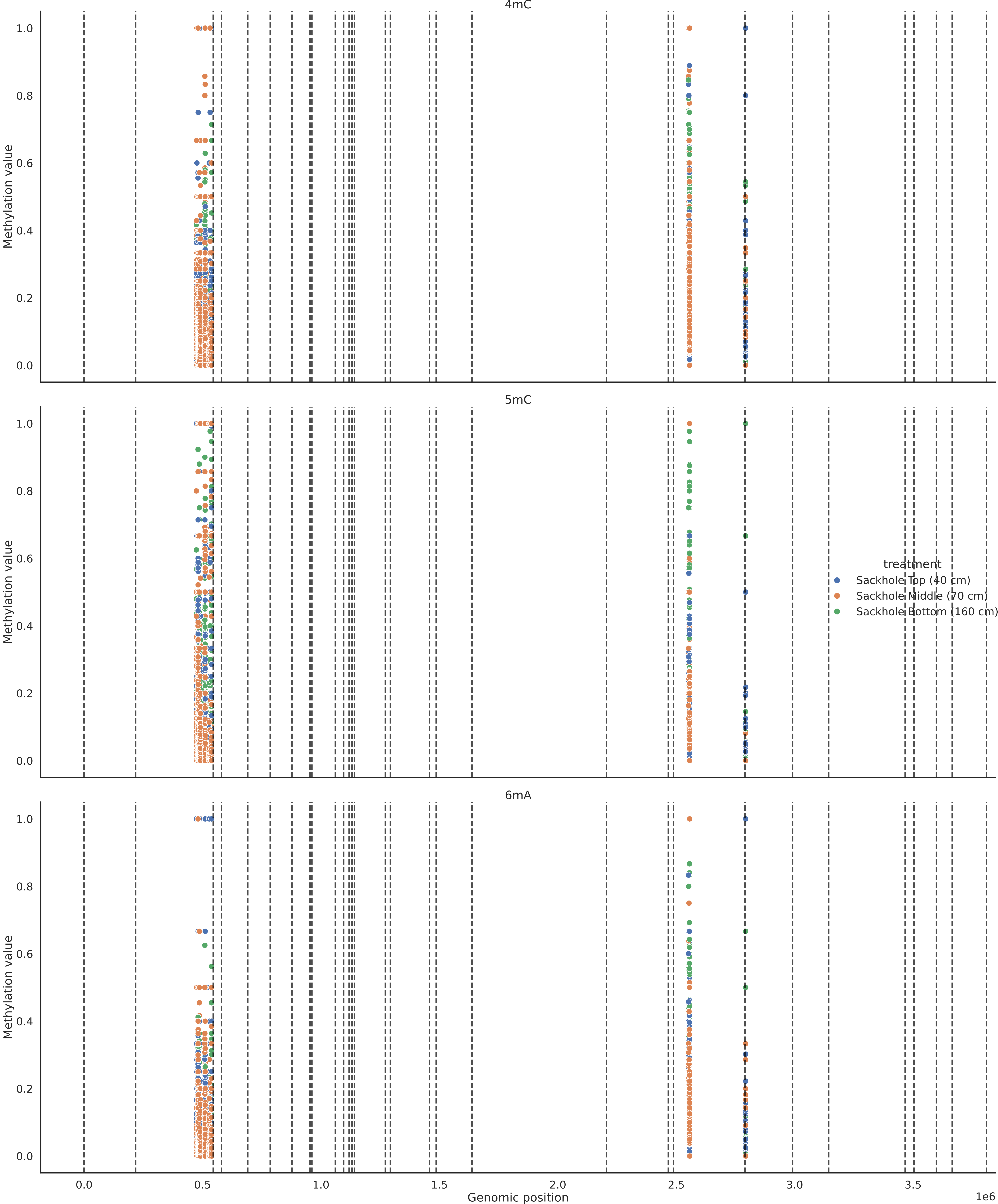
Methylation value across genome of common positions in Octadecabacter sp. coverage 5
