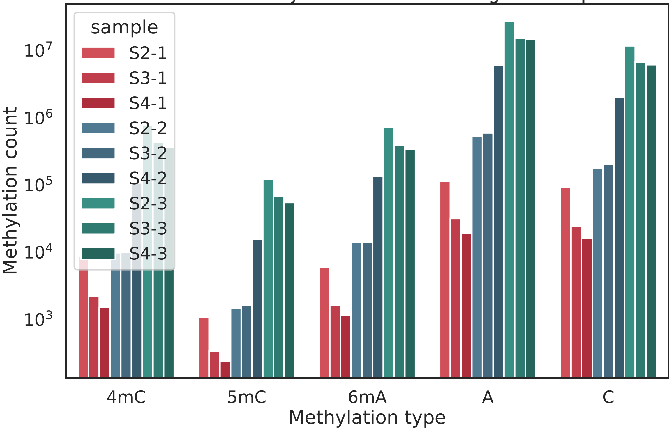
Number of methylation counts in Pelagibacter sp.
