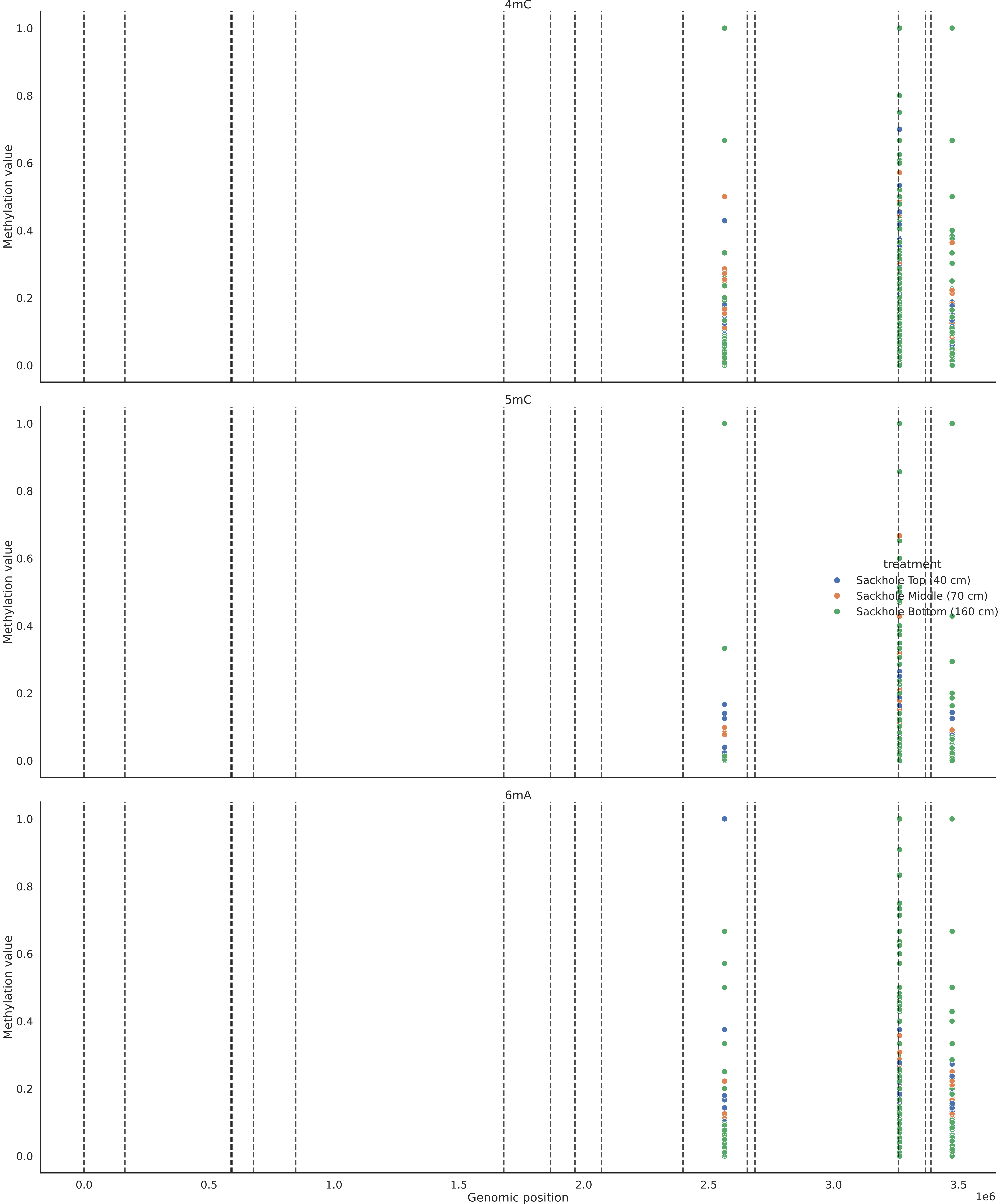
Methylation value across genome of common positions in Brevundimonas sp. coverage 6
