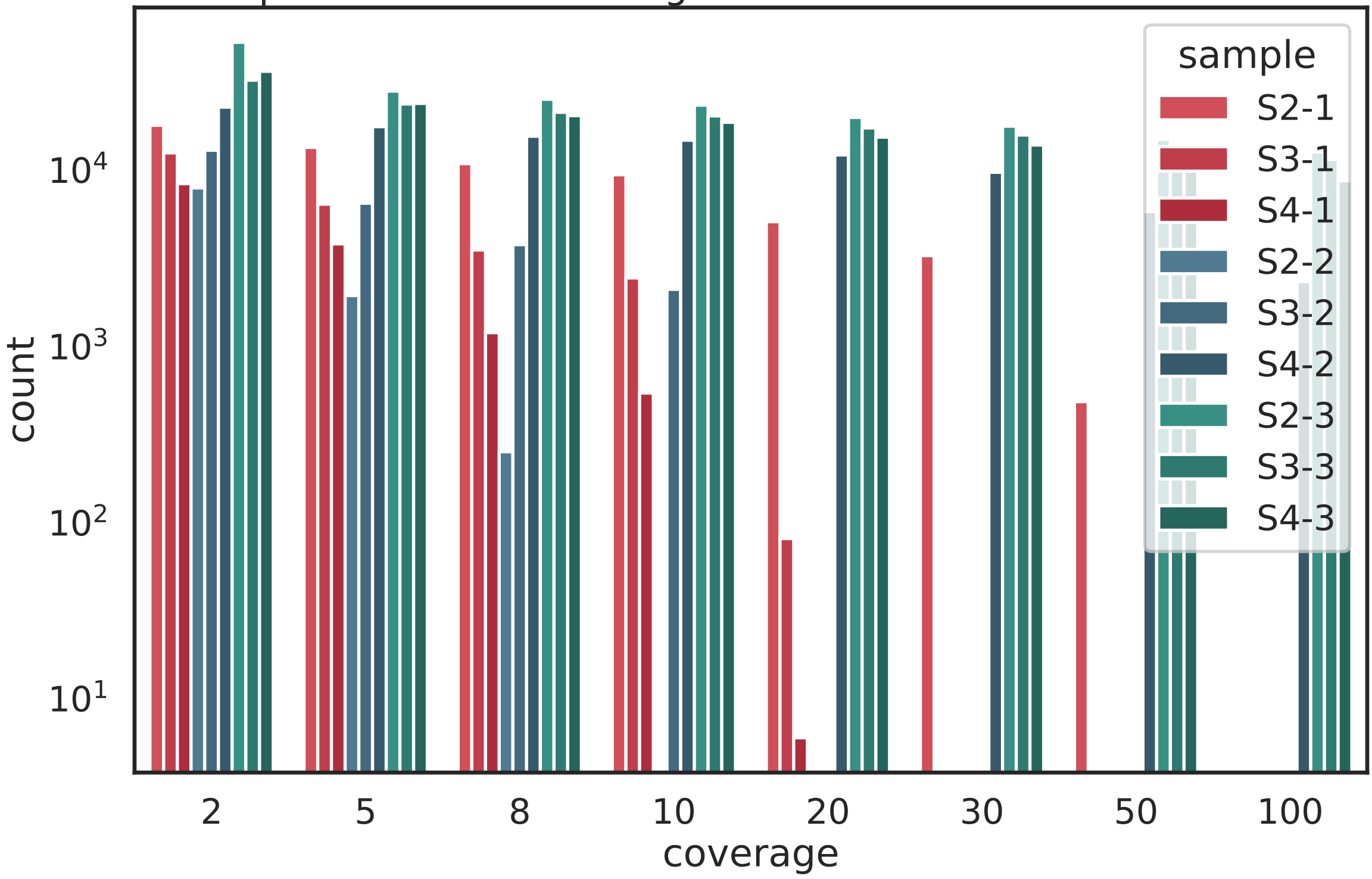
Number of positions with coverage above threshold in Brevundimona
