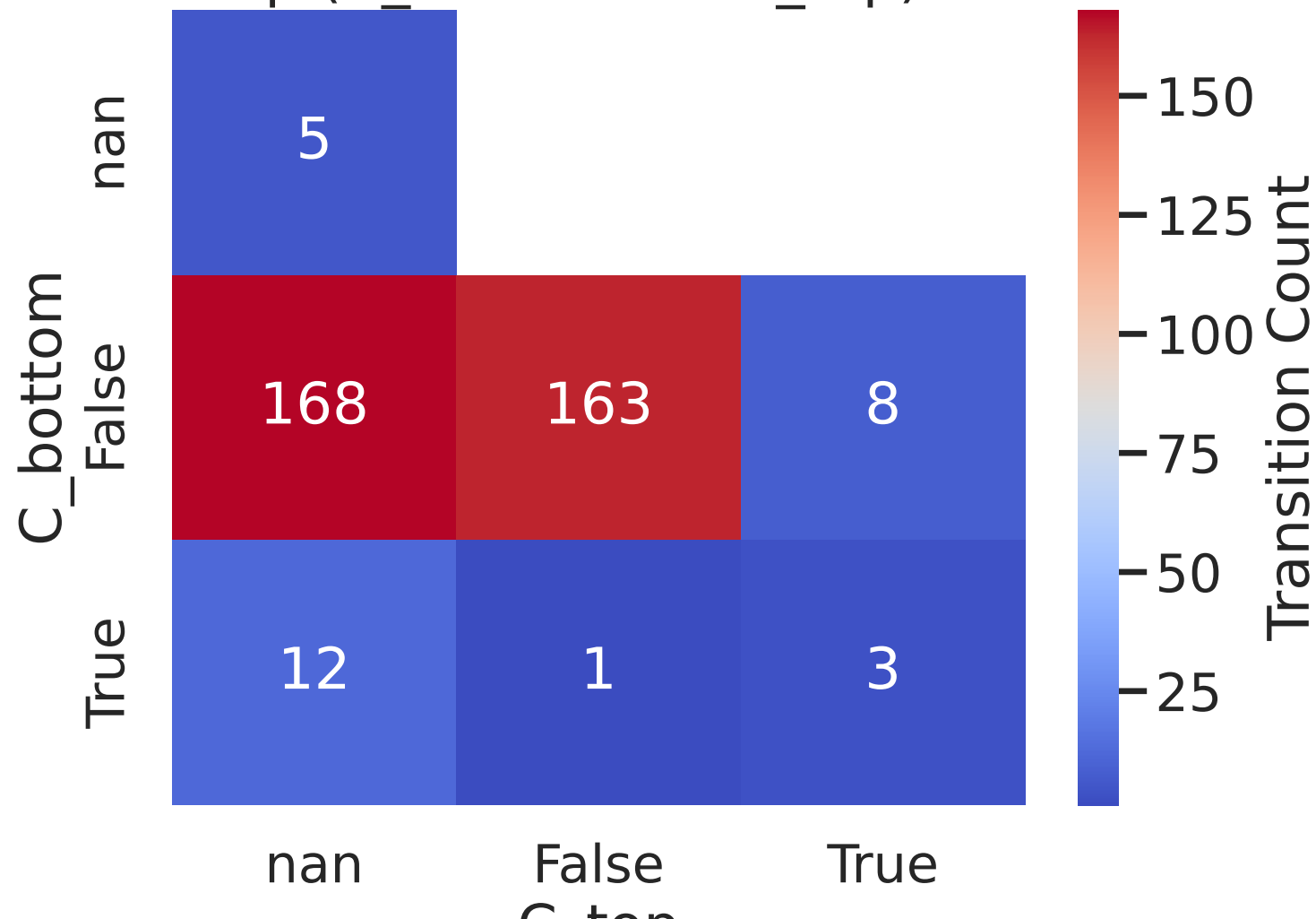
Heatmap (C_bottom vs. C_top) in Polaribacter
