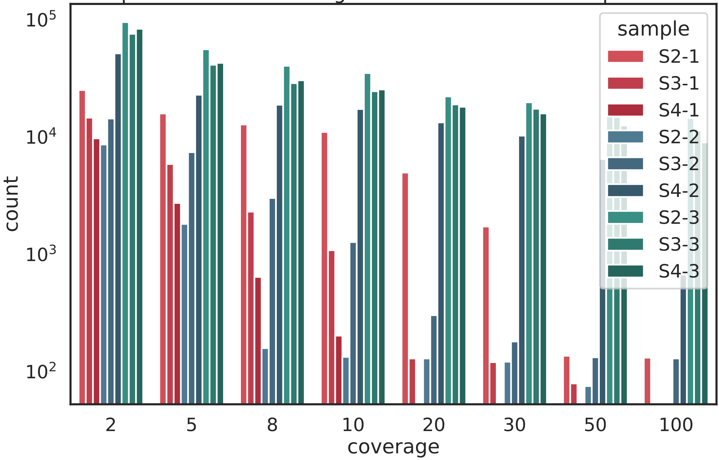
Number of positions with coverage above threshold in Halopseudomon
