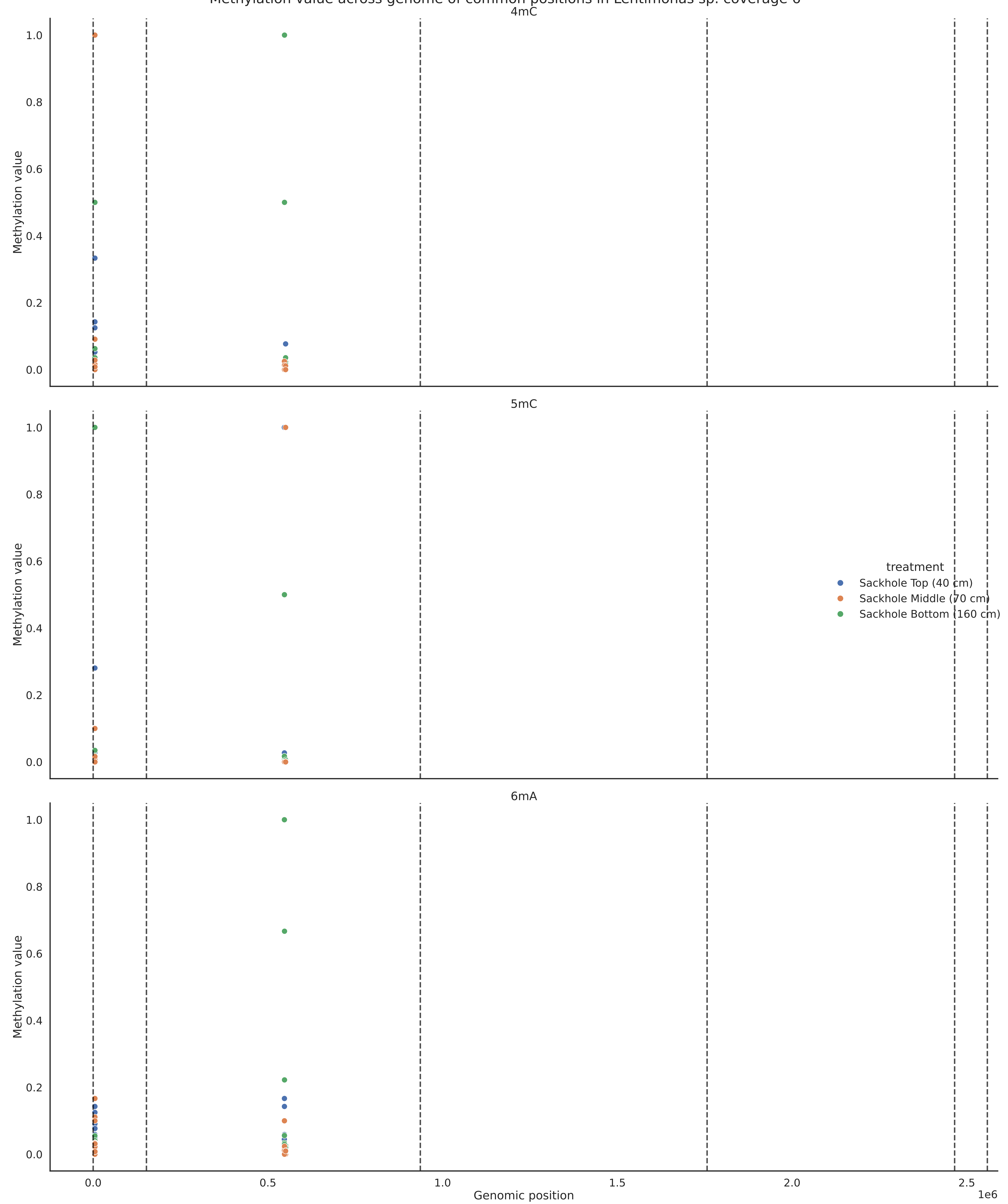
Methylation value across genome of common positions in Lentimonas sp. coverage 6
