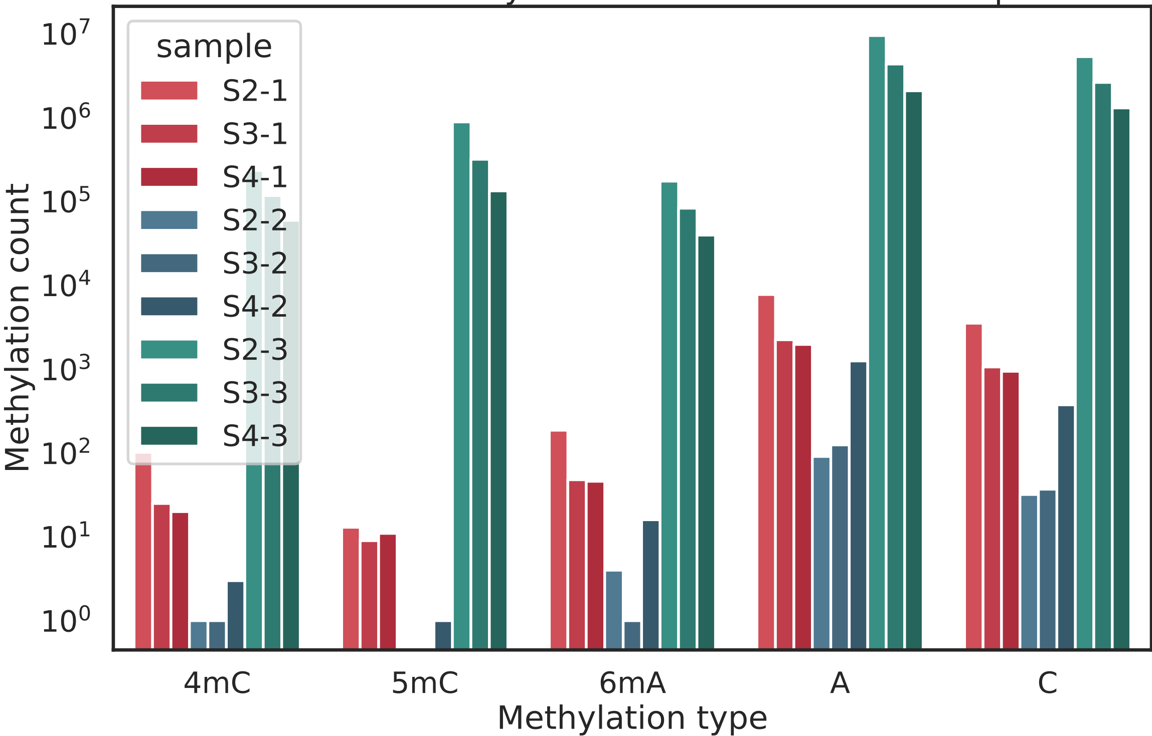
Number of methylation counts in Lentimonas sp.
