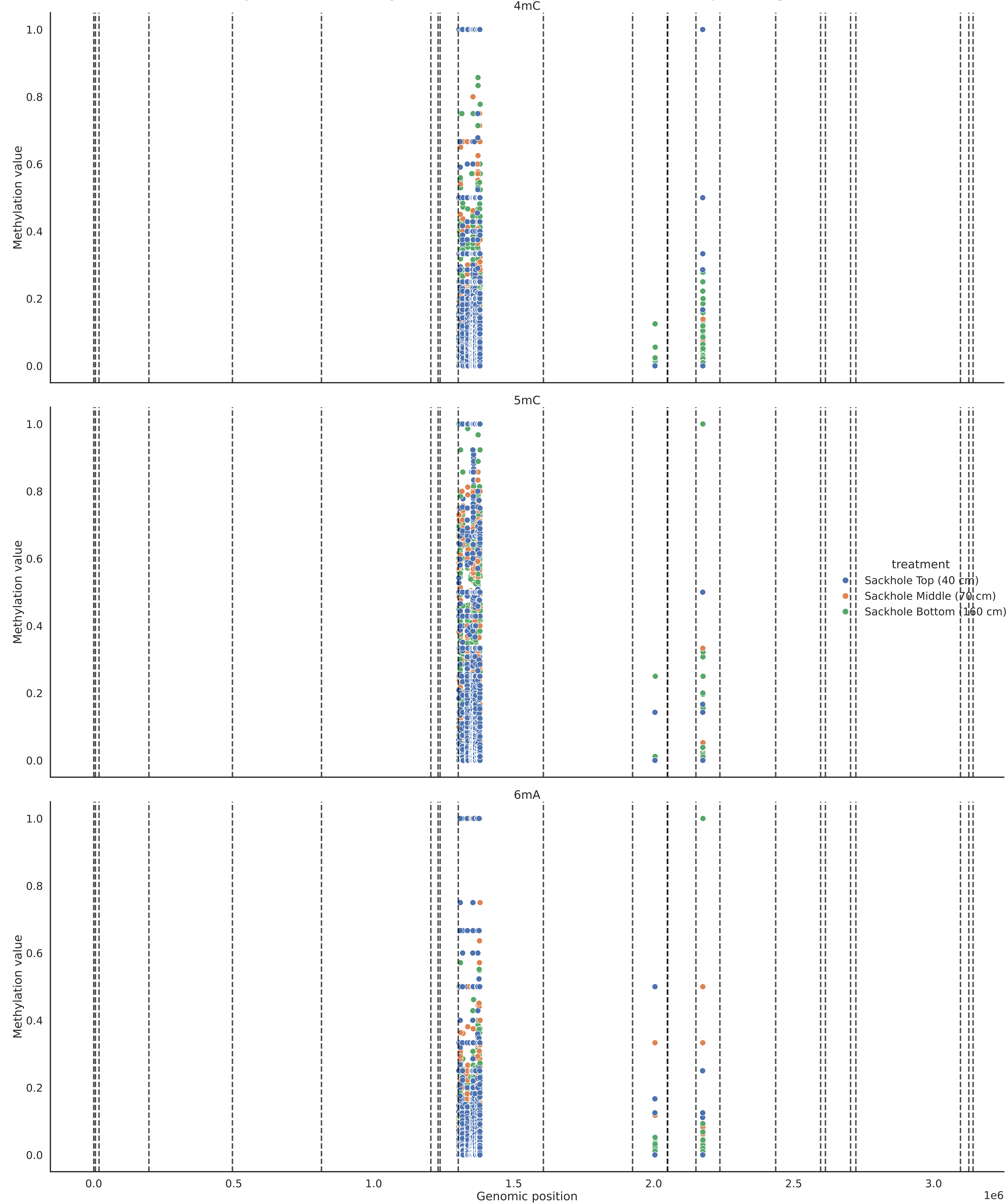
Methylation value across genome of common positions in Polaribacter sp. coverage 2
