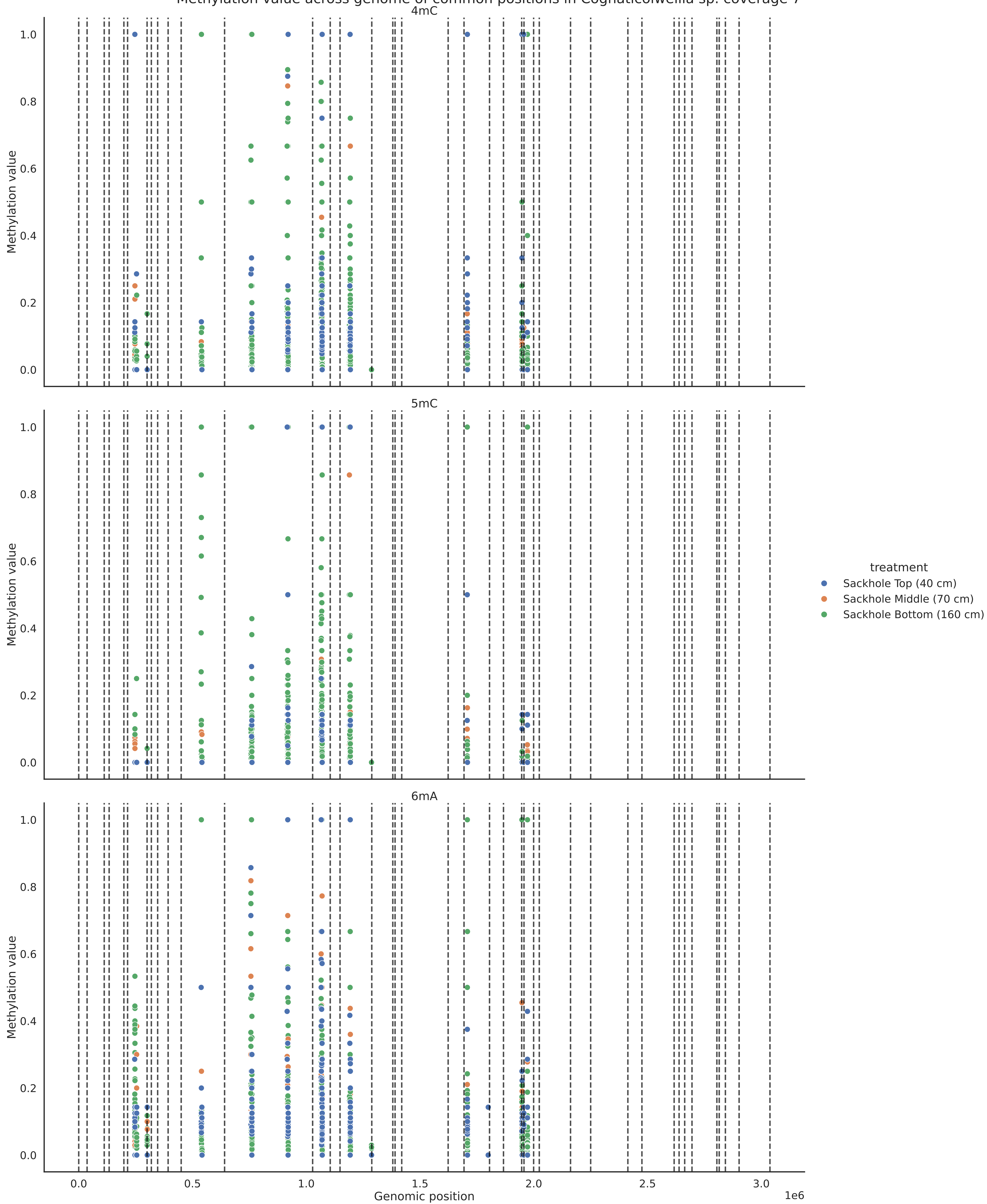
Methylation value across genome of common positions in Cognaticolwellia sp. coverage 7
