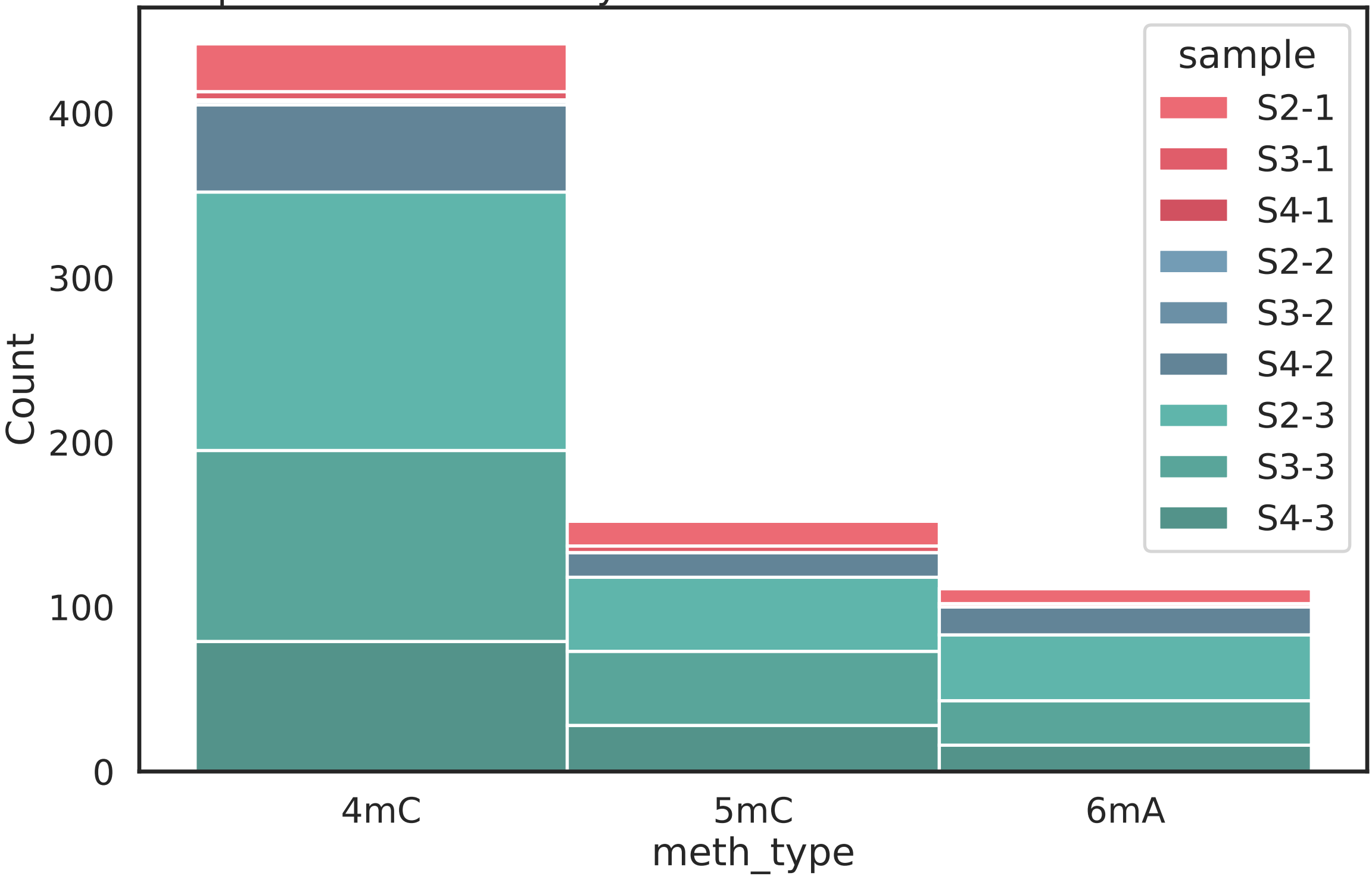
Number of positions 95% methylated in all 3 treatments in Brevundimono
