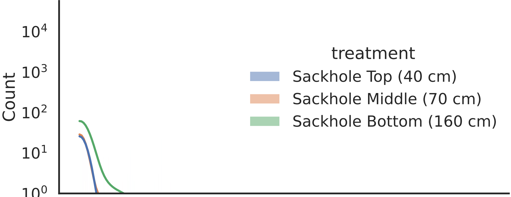
5mC distribution
