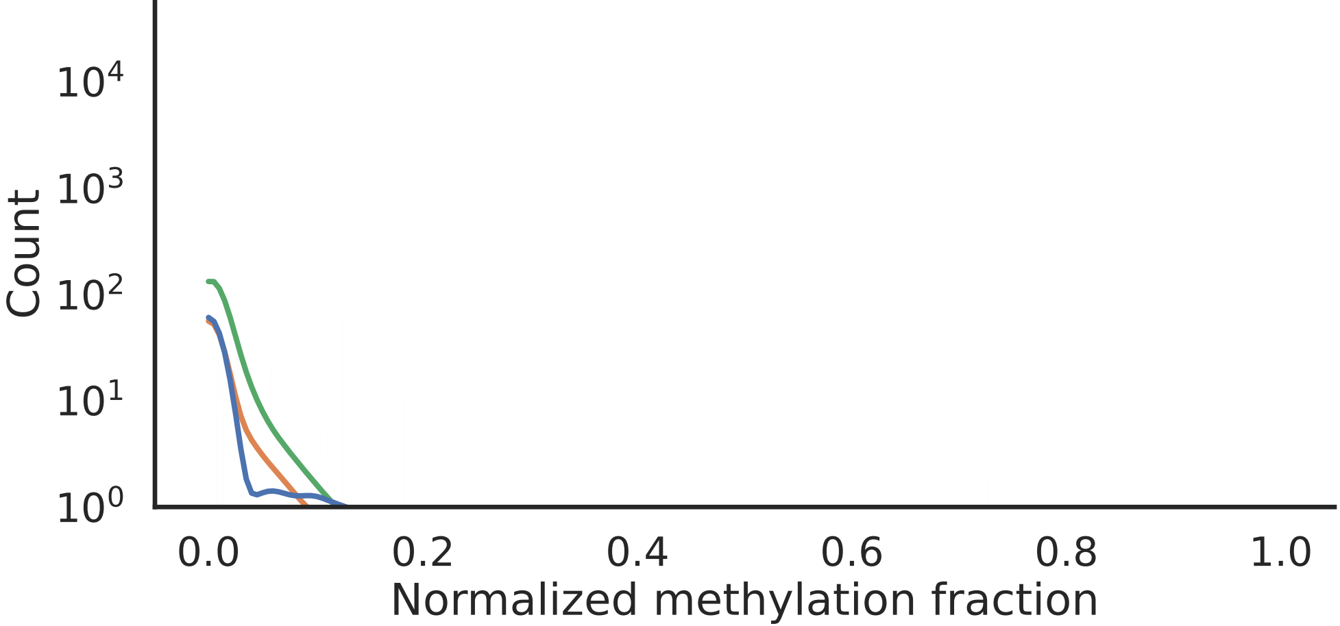
6mA distribution
