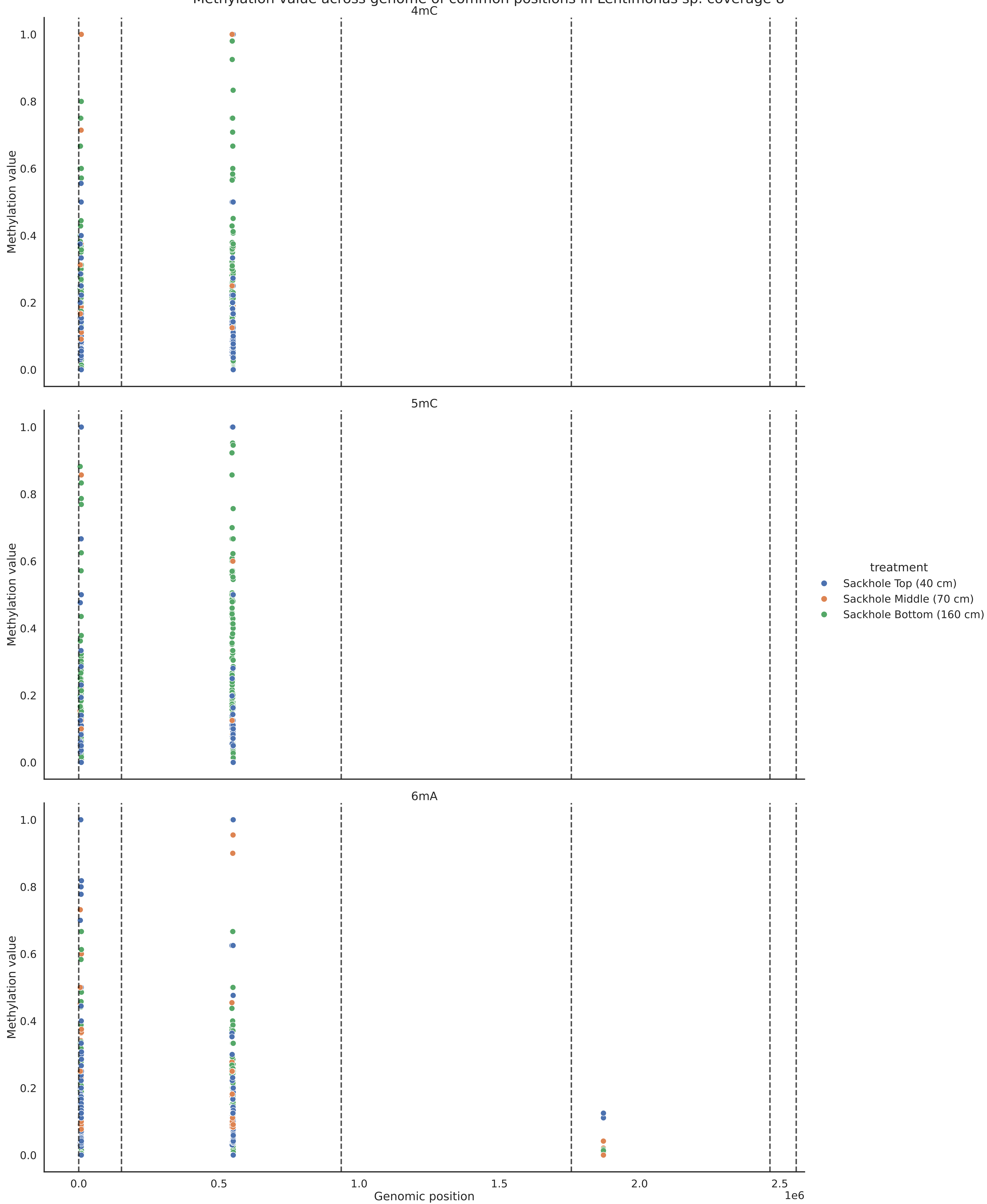
Methylation value across genome of common positions in Lentimonas sp. coverage 8
