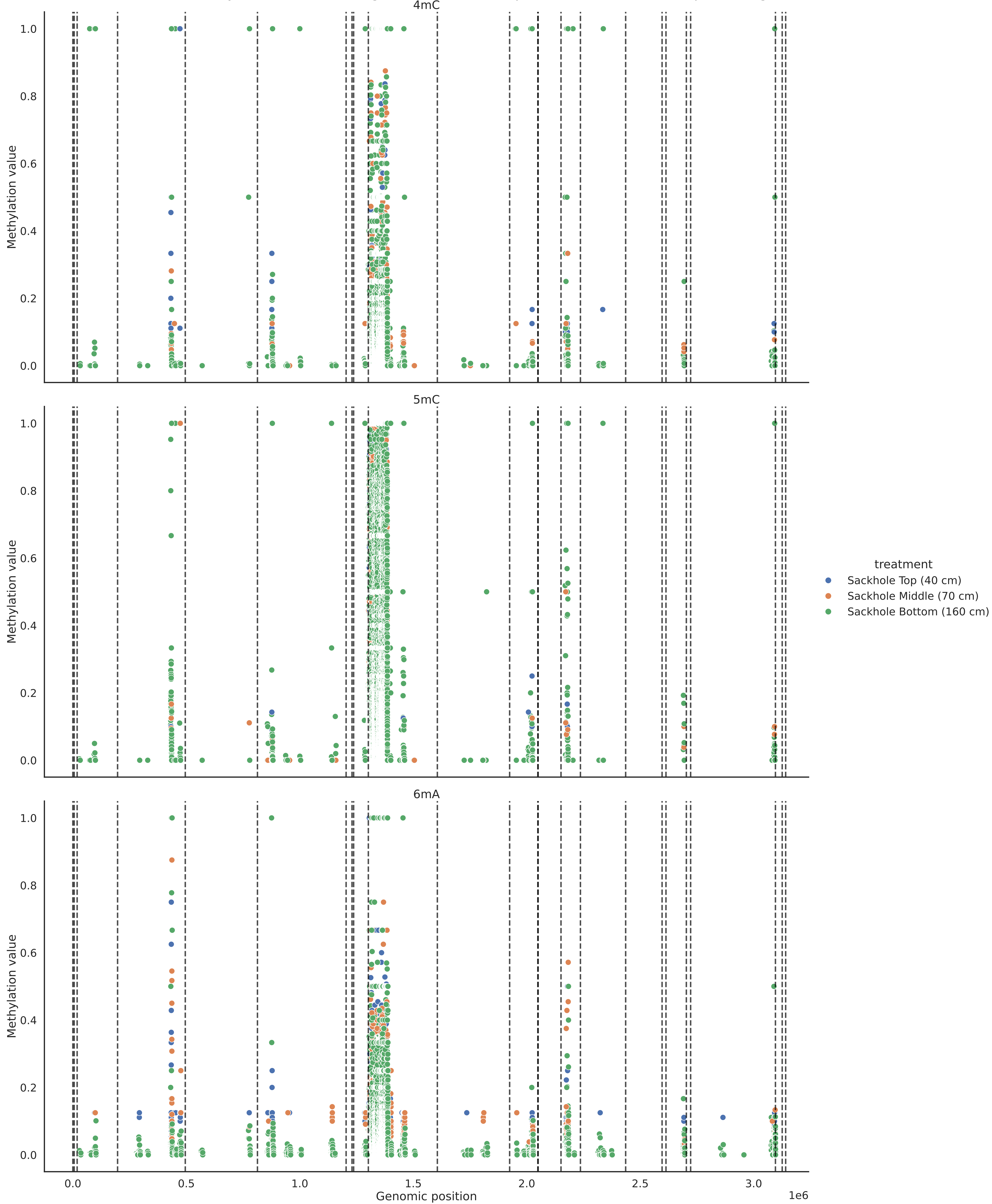
Methylation value across genome of common positions in Polaribacter sp. coverage 8
