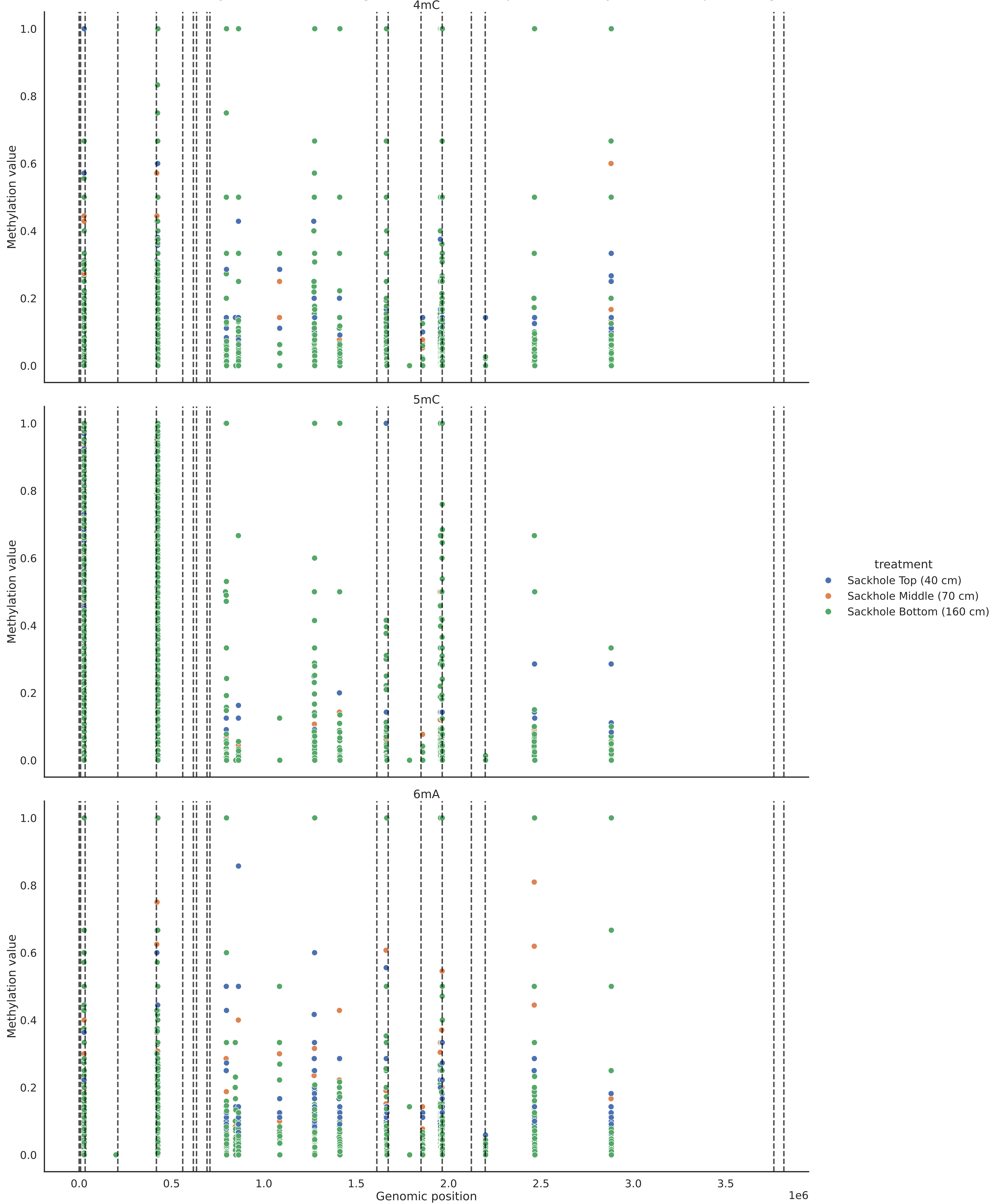
Methylation value across genome of common positions in Psychromonas sp. coverage 7
