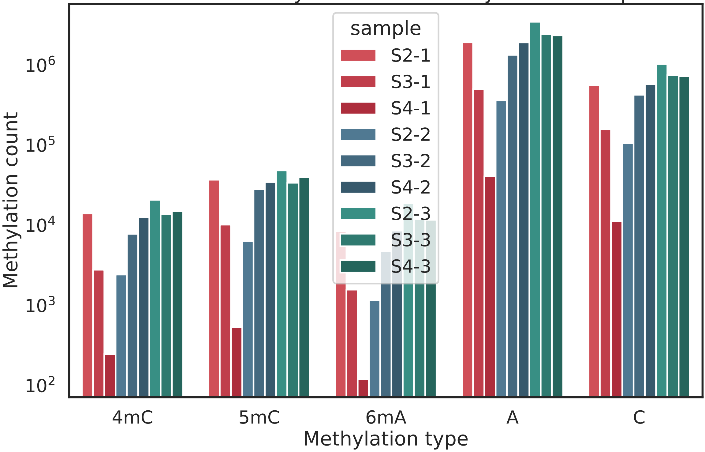
Number of methylation counts in Psychromonas sp.
