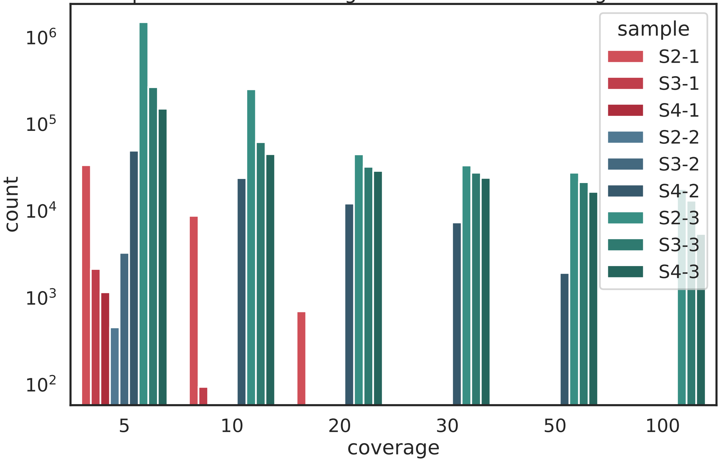
Number of positions with coverage above threshold in Cognaticolwelli
