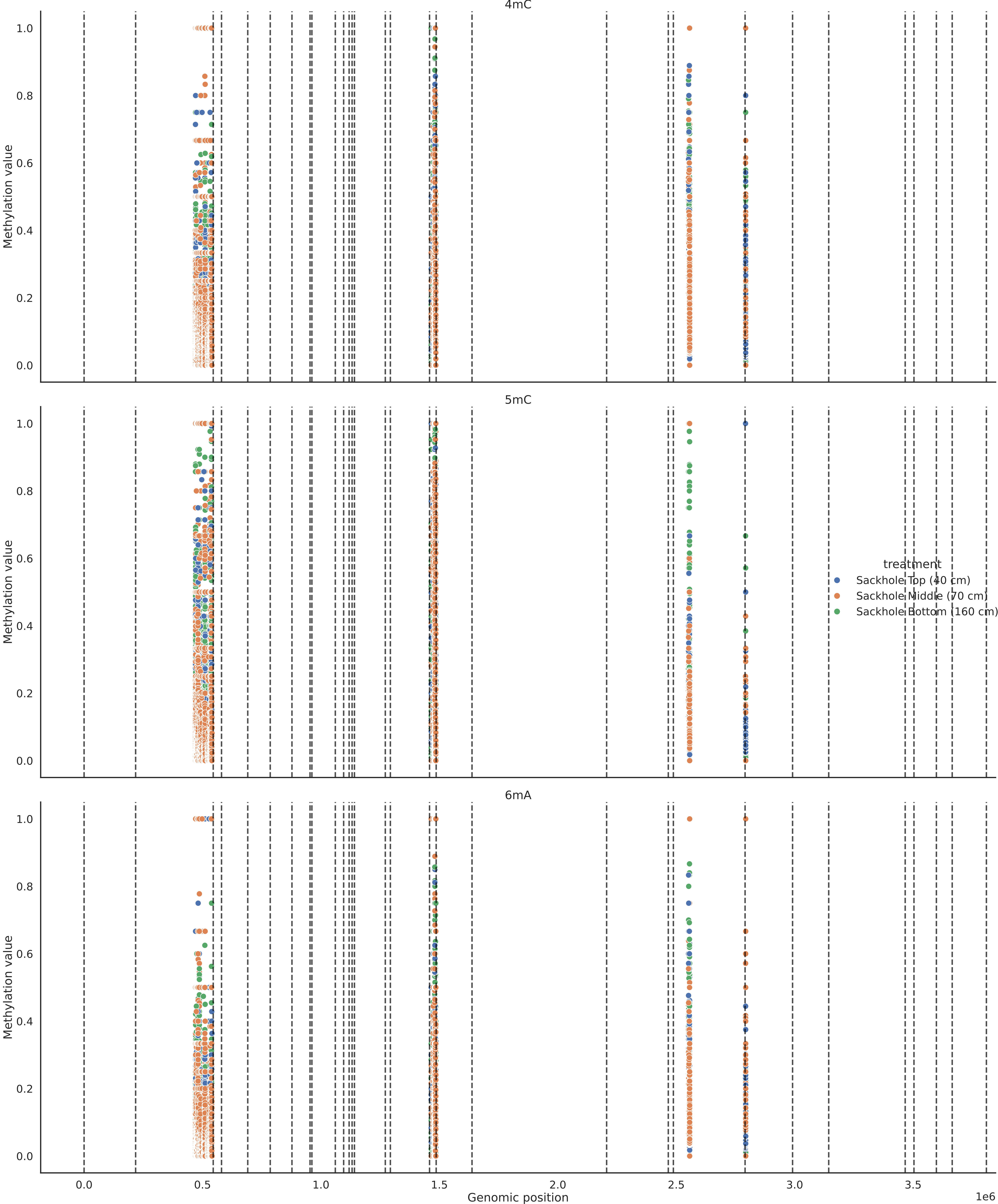
Methylation value across genome of common positions in Octadecabacter sp. coverage 2
