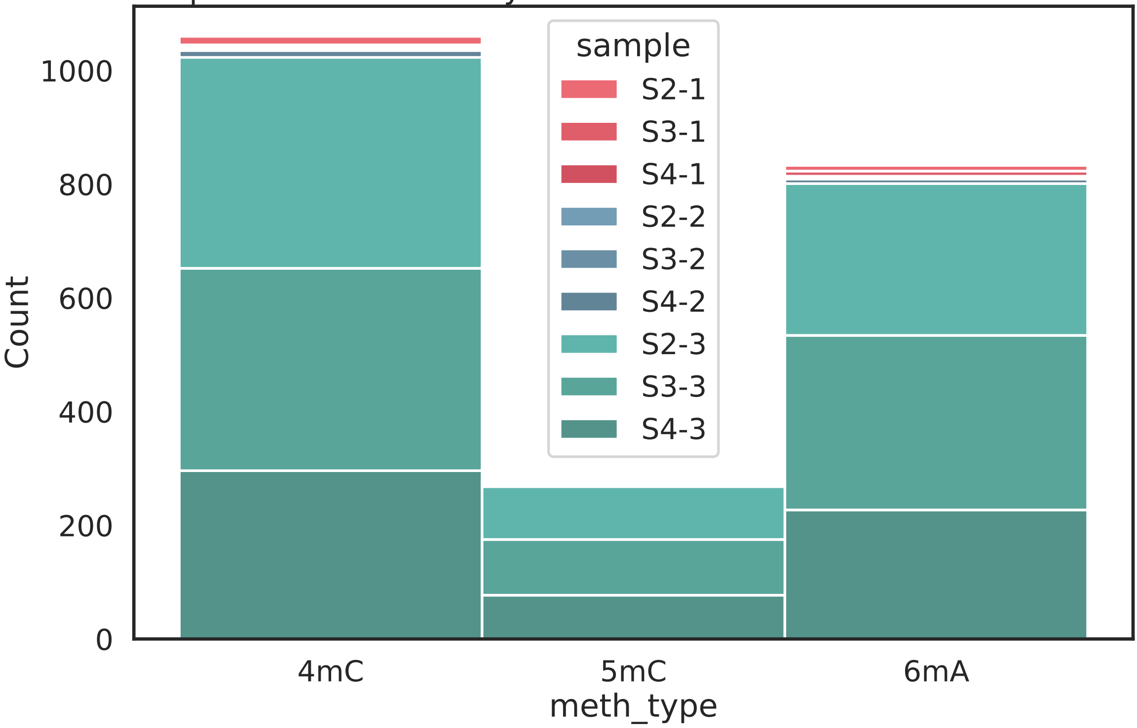
Number of positions 95% methylated in all 3 treatments in Brevundimor
