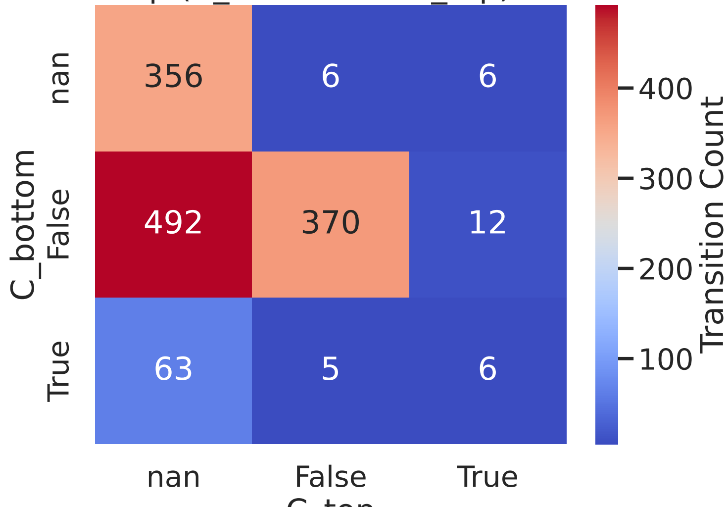
Heatmap (C_bottom vs. C_top) in Lentimonas s
