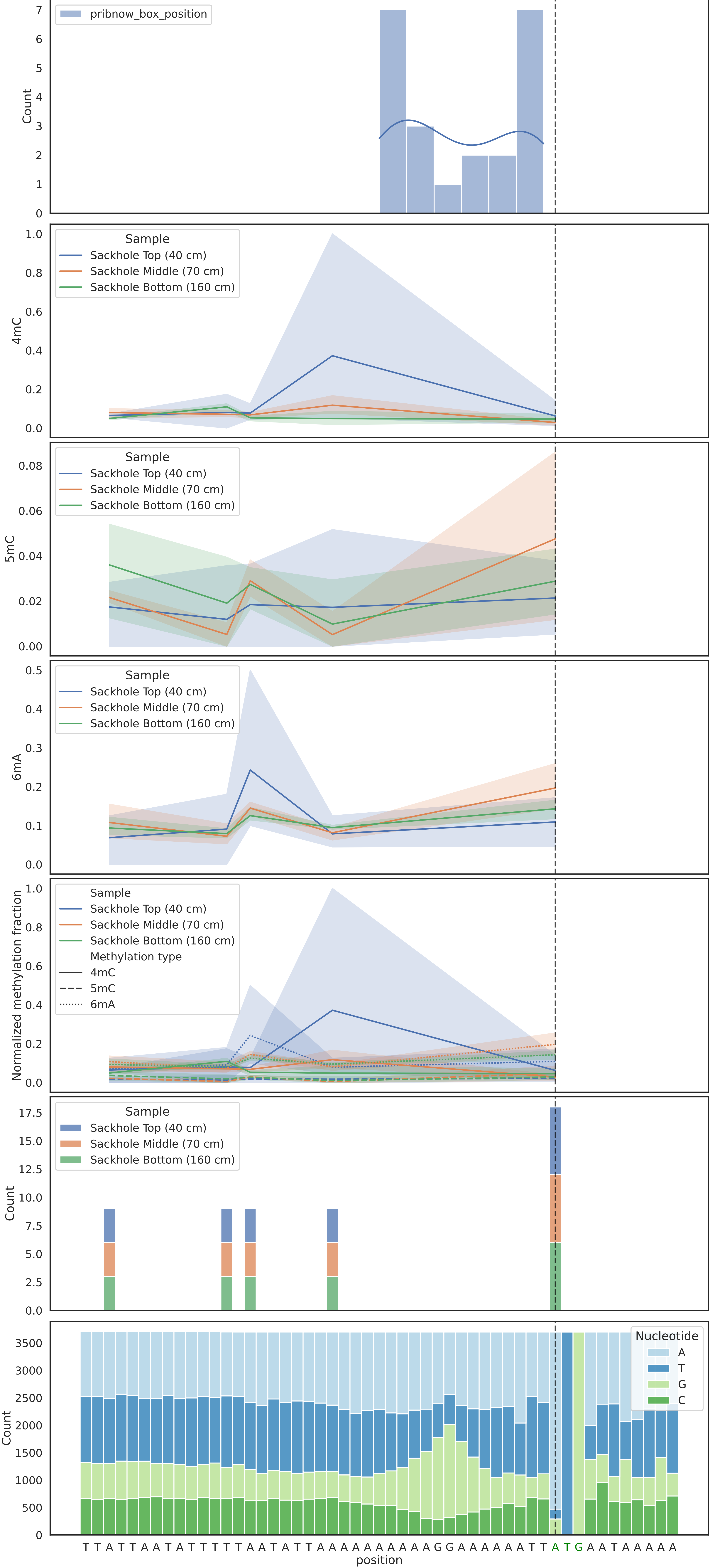
All gene promoter methylation in Psychromonas sp. Proportion of genes with pribnox box: 22 / 3708
