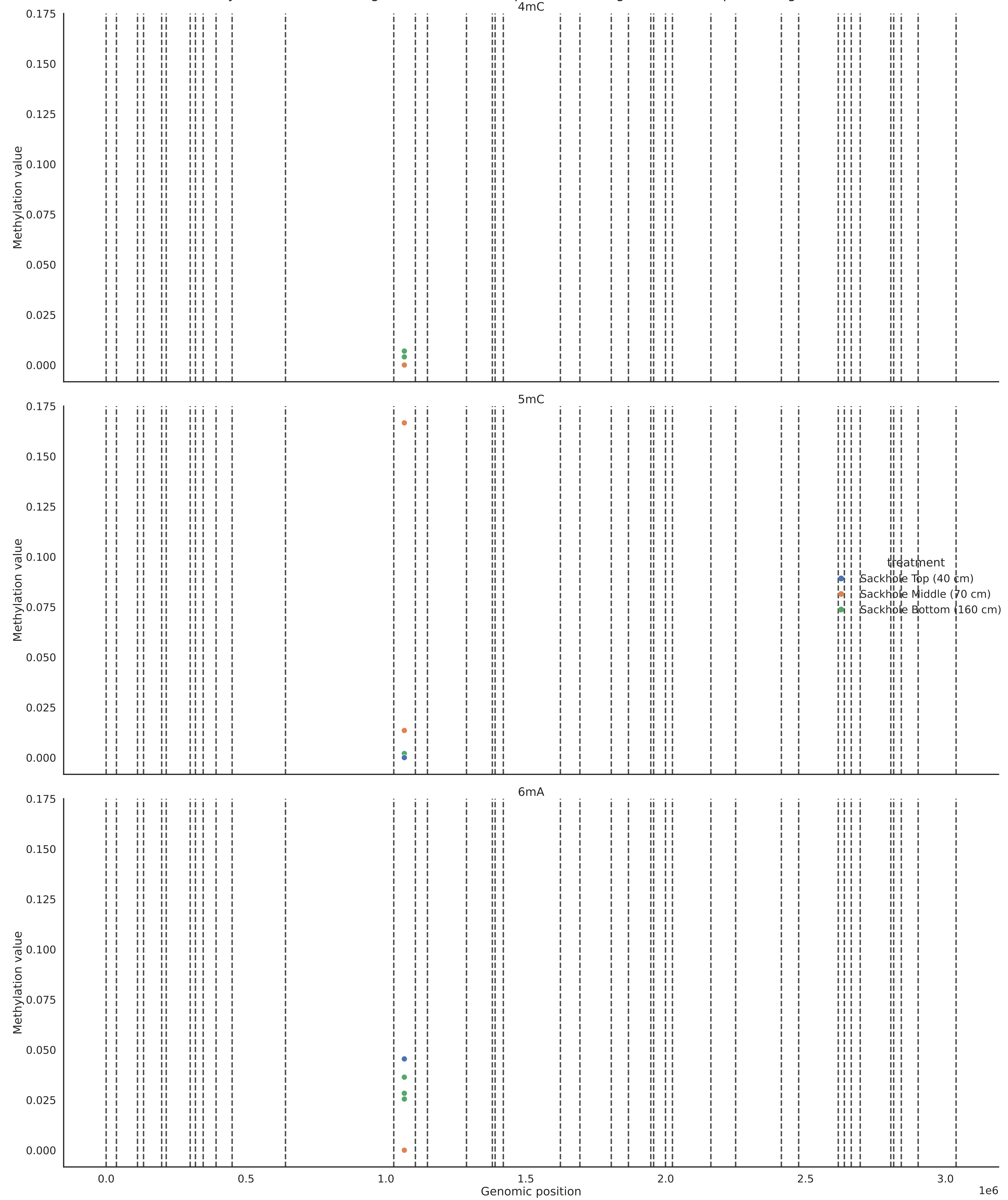
Methylation value across genome of common positions in Cognaticolwellia sp. coverage 6
