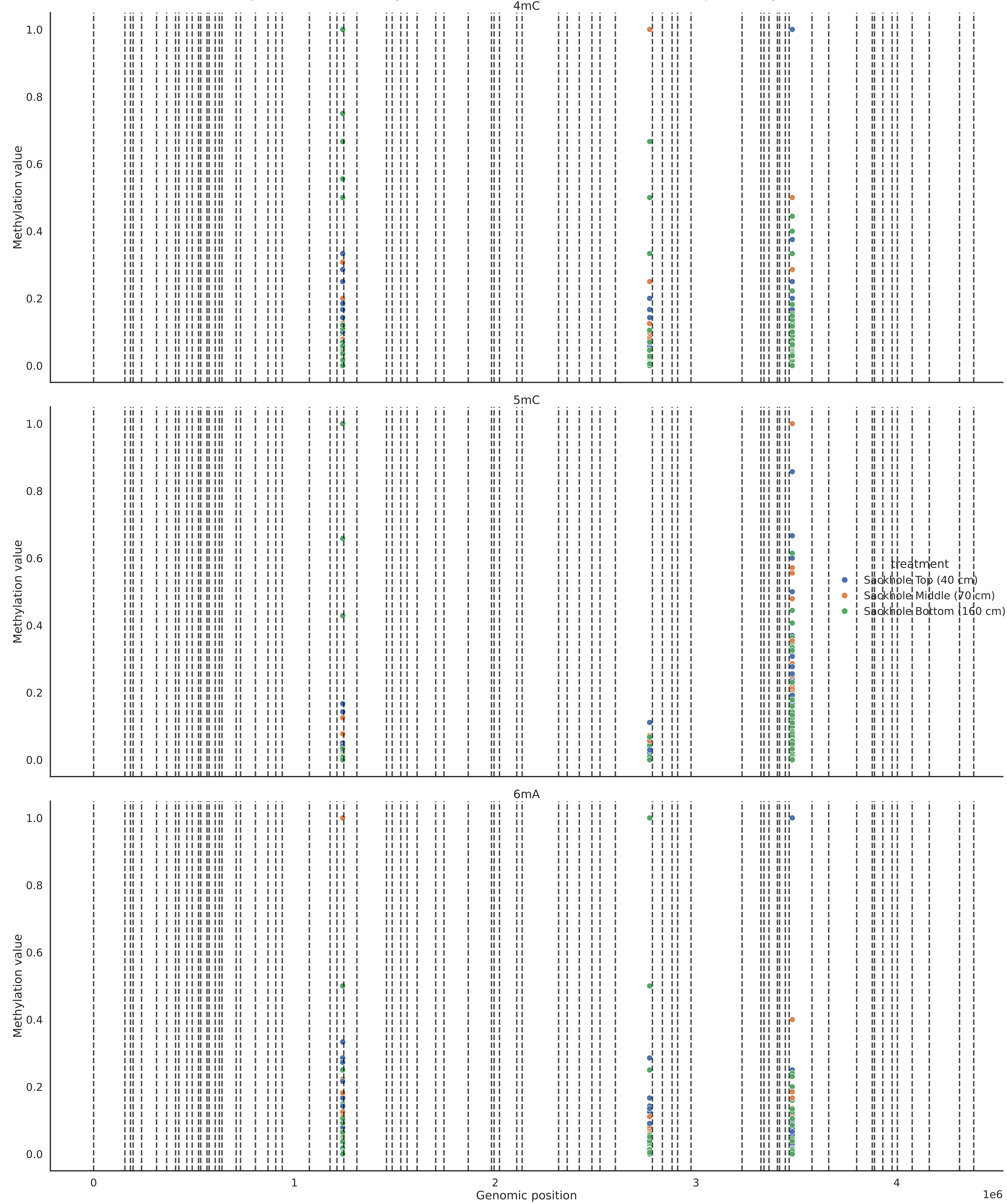
Methylation value across genome of common positions in Rubritalea sp. coverage 6
