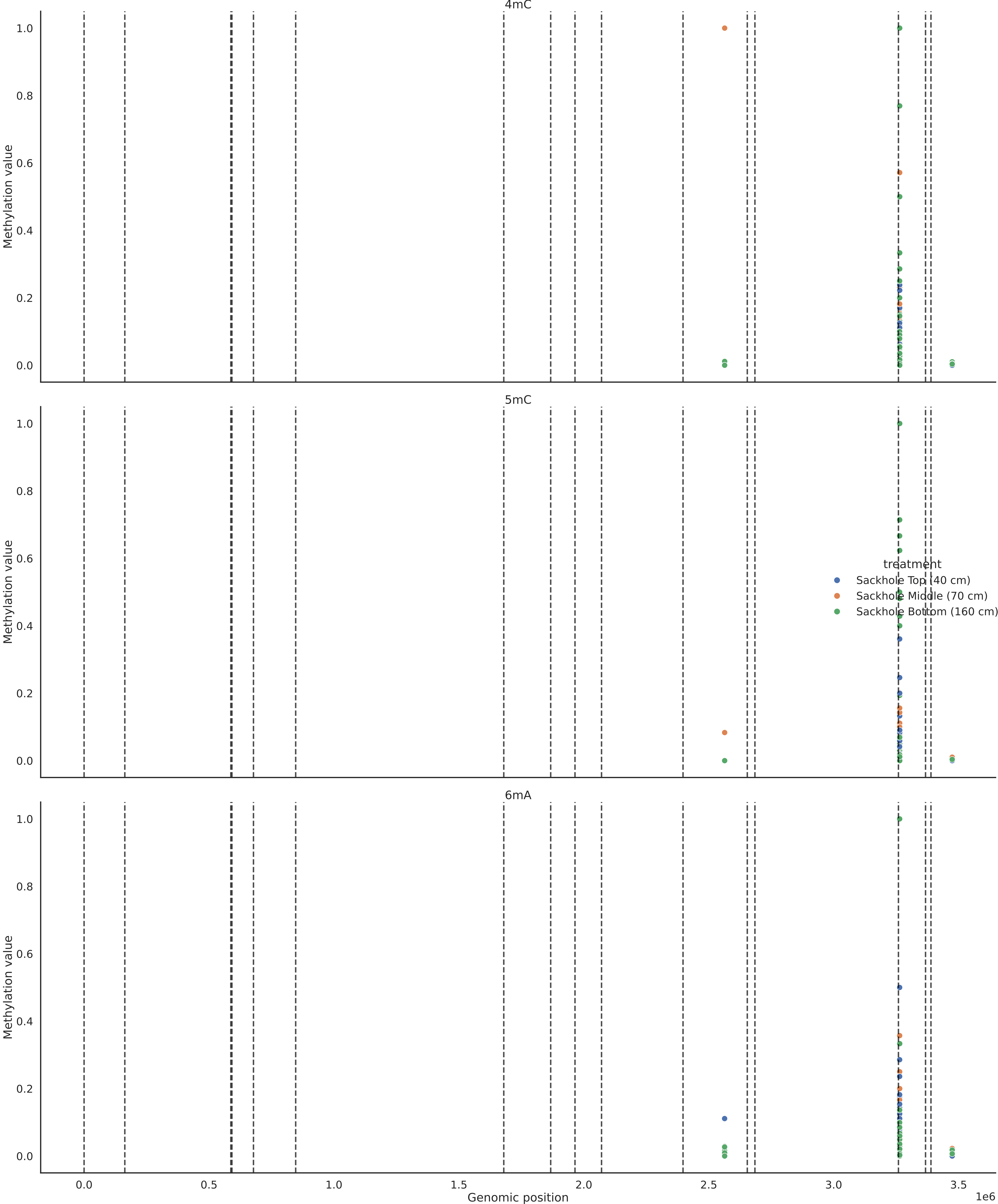
Methylation value across genome of common positions in Brevundimonas sp. coverage 7
