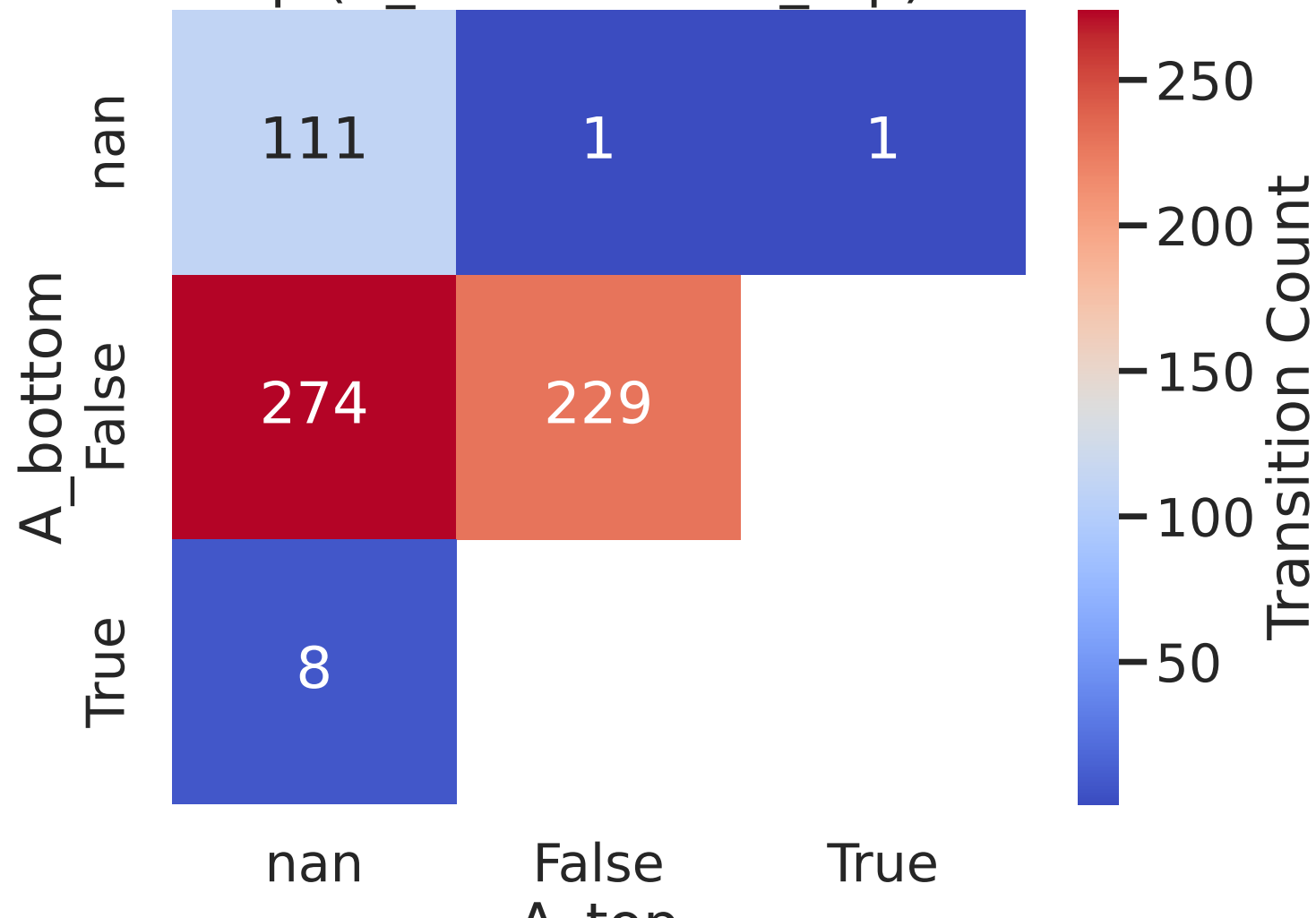
Heatmap (A_bottom vs. A_top) in Lentimonas s
