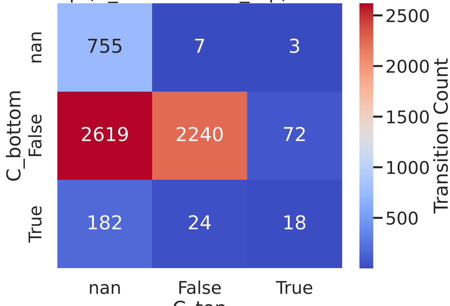
Heatmap (C_bottom vs. C_top) in Octadecabacter
