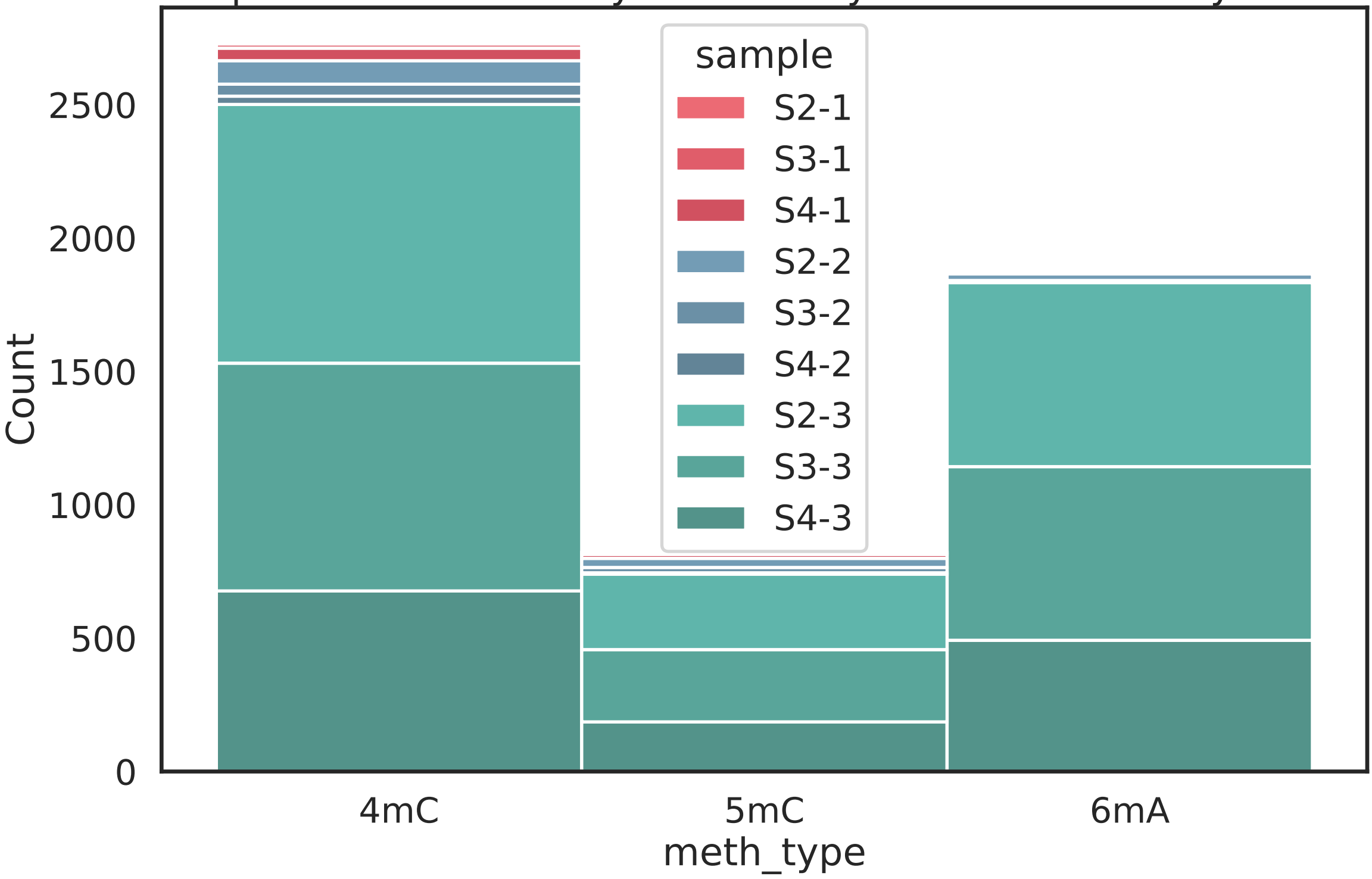
Number of positions 95% methylated in only 1 treatment in Psychromono
