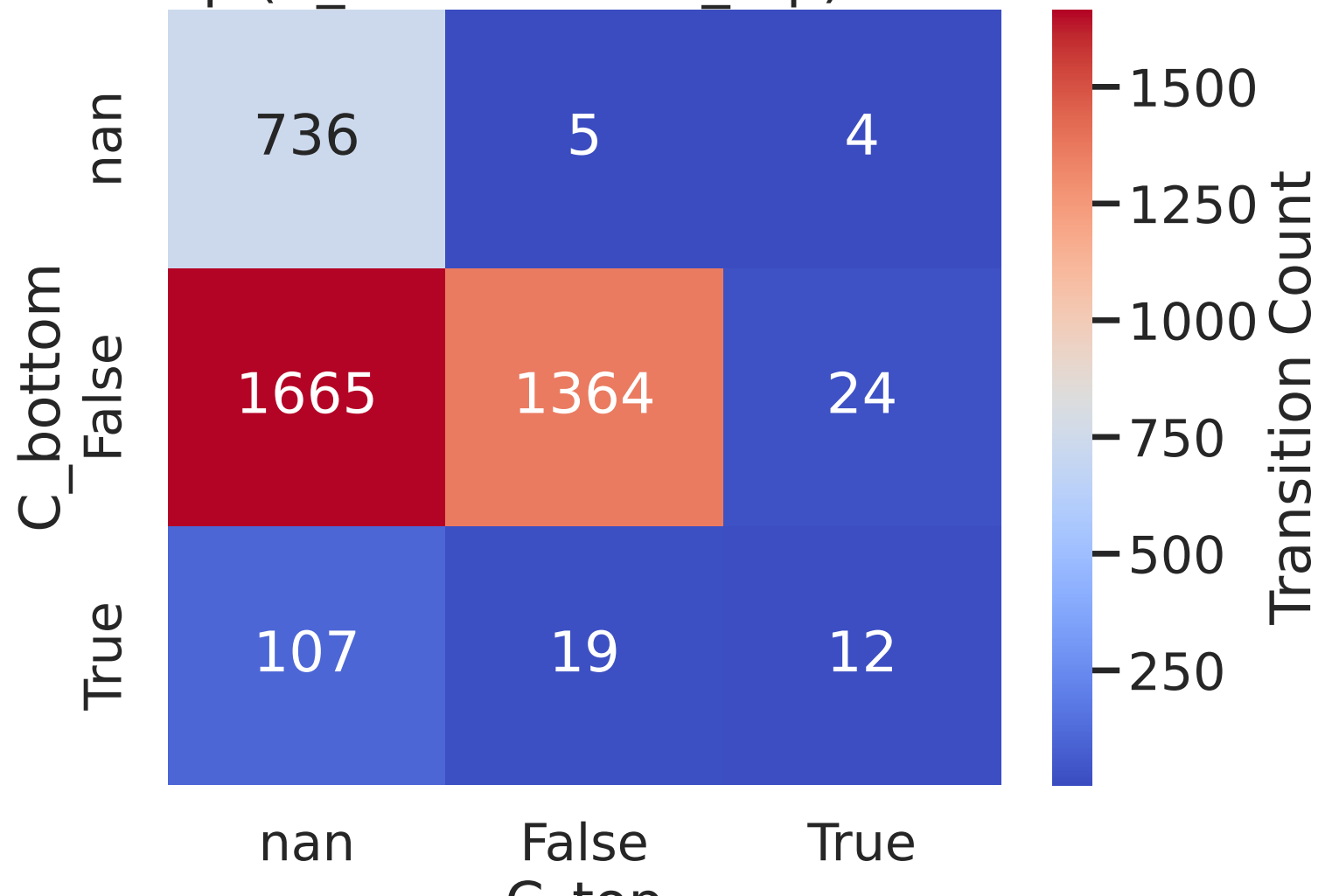
Heatmap (C_bottom vs. C_top) in Octadecabacte
